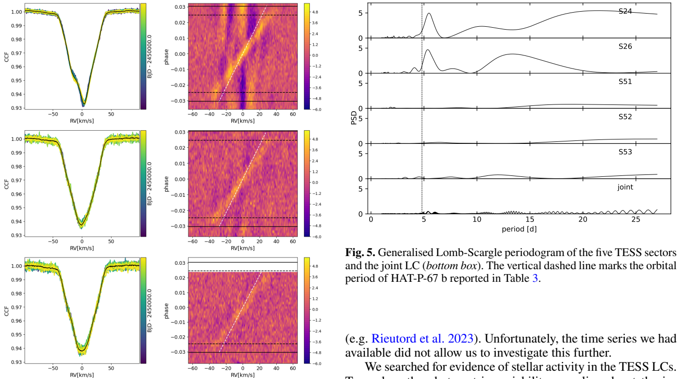
Fig. 4. Cross-correlation function for N1 (first row), N3 (second row), and N4 (third row) extracted from the DRS using a G2 mask. Left: cross-correlation function linear profiles as a function of time. The black line indicates the average CCF. Right: two-dimensional maps of the CCFs as a function of orbital phase and RV in the stellar rest frame. The four horizontal black lines show the times of transit contacts. The straight white line shows the expected planetary Keplerian velocity K_p using a planetary mass value of \sim 0.34 M_J (Zhou et al. 2017).
