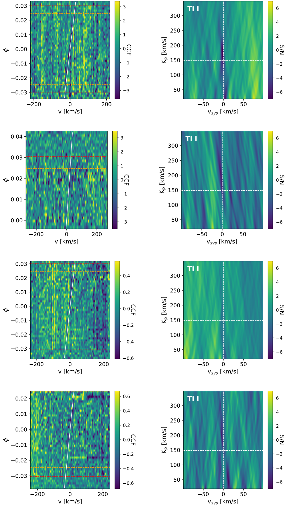
Fig. A.5: Same as Figure A.2 but for the Ti I mask.
