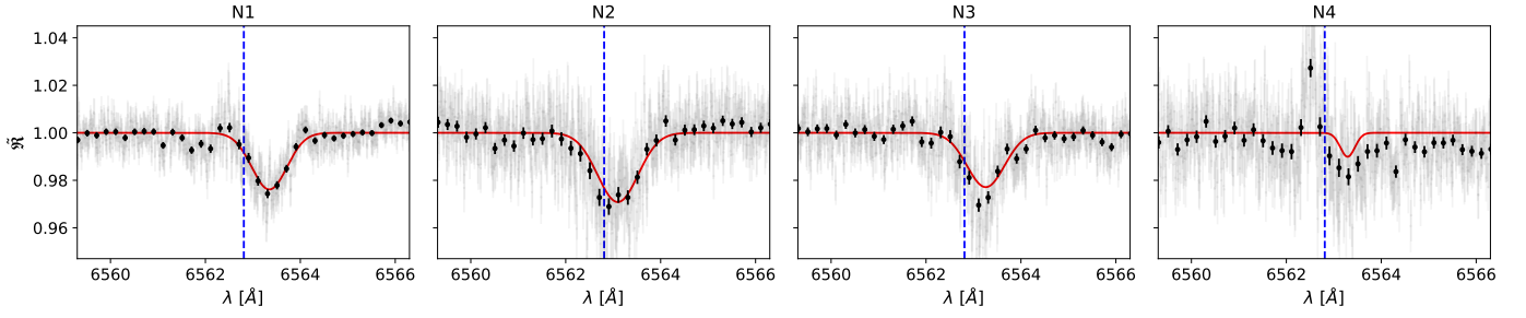
Fig. 8. Transmission spectra of HAT-P-67 b for each night. The spectra are centred around the H \alpha line in the planetary rest frame (light grey) and also binned 20 times (in black circles). The red line is the MCMC Gaussian fit performed by SLOppy, while the vertical blue dashed line indicates the rest frame transition wavelength of the H \alpha line.
