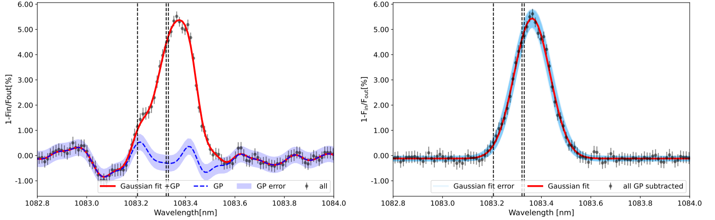
Fig. A.9: Gaussian process correction. Right panel: Transmission spectrum centred on the He I triplet (in the planet rest frame) with the GP regression model overplotted and with the 1\sigma uncertainty intervals (in blue) and the Gaussian+GP model (in red). Left panel: Final transmission spectrum after removing the GP model. The error intervals for the Gaussian fit were computed by displaying 1000 Gaussian fits within the 1\sigma uncertainties of the derived parameters spanning the 16%-84% quantiles. Vertical black dotted lines indicate the position of the He I triplet.
