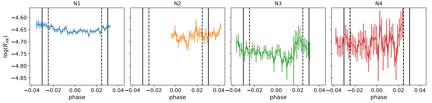
Fig. 3. Activity indicator \log R'_{HK} as a function of the time for each night. The continuous black lines indicate the points of first and fourth contact of the transit, while the dashed black lines represent the points of second and third contact.
