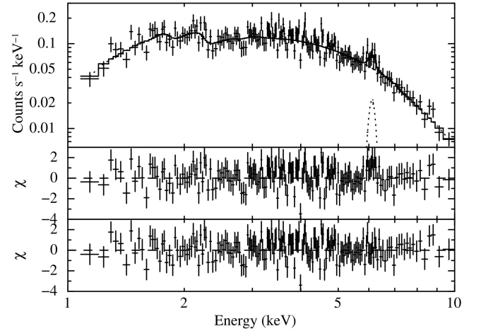
Fig. 5. EPIC spectrum of CXOU J225355.1+624336 corresponding to phase range A. Upper panel: overlap of the spectrum with the best-fitting TBPCF×(PL+Gaussian) emission model, where the Gaussian component is shown. Middle panel: data-model residuals, in units of standard deviation ( \sigma ), in the case of the best-fitting TBPCF×PL model. Lower panel: data-model residuals, in units of standard deviation ( \sigma ), in the case of the best-fitting TBPCF×(PL+Gaussian) model.
