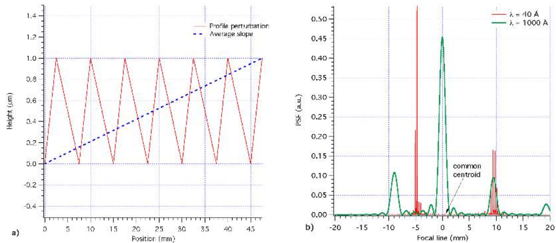
Figure 2. Left: An asymmetric figure error in the mid-frequency range. Right: The PSF computed in UV light ( \lambda = 100 \text{ nm} ) and X-rays ( \lambda = 1 \text{ nm} ). Both PSFs were computed using the WISE code [1] . As expected, the centroid was displaced near x = 1 \text{ mm} . Even if the perturbation has a much higher relevance at high energy, and therefore two PSFs look completely different in the two cases, the centroid position is the same.
