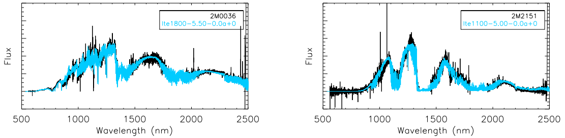
Figure 2: Best matches to BT-Settl models 2014. Effective temperature, gravity, metallicity and alpha element enhancement are described in the model name strings as lte-LOGG+[M/H]a+[ALPHA/H] . The flux is F(\lambda) .
