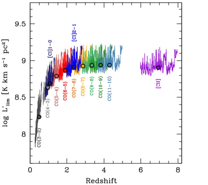
Figure 1. Sensitivity limits of the ASPECS 1.2 mm cube. Left: channel rms as a function of frequency. For a 15.6 MHz channel, the typical rms is \sim 0.5 mJy beam ^{-1} throughout the entire band. The frequency settings used in the observations (labeled A–H) and the edges of each spectral window are also marked. Right: line luminosity limits (in units of K km s ^{-1} pc ^2 ) as a function of redshift. Here we assume a 5\sigma limit for a line width of 200 km s ^{-1} . The dots highlight the fiducial limit, obtained as the median sensitivity throughout the band.
