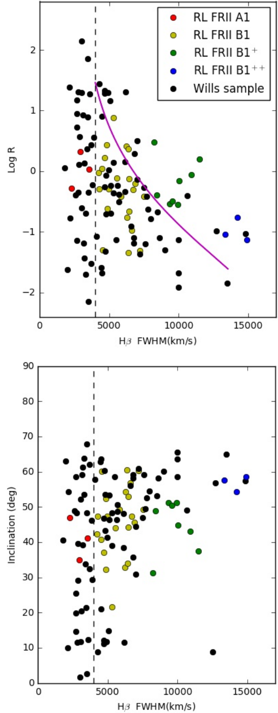
Fig. 13. Top: core-to-lobe radio flux density ratio vs. \text{FWHM}(H\beta) , adapted from Wills & Browne (1986) . Colored dots represent sources of our sample: red dots represent A1 RL FR II sources, yellow dots B1 RL FR II, green B1 + RL FR II and blue ones B1 ++ RL FR II. Black dots are the original data from Wills & Browne (1986) . The magenta line represents the change of R with \text{FWHM}(H\beta) , predicted by the Orr & Browne (1982) beaming model with R_T = 0.024 and \gamma = 5 . Bottom: \text{FWHM}(H\beta) vs. inclination, derived from R_c through Eq. (16).
