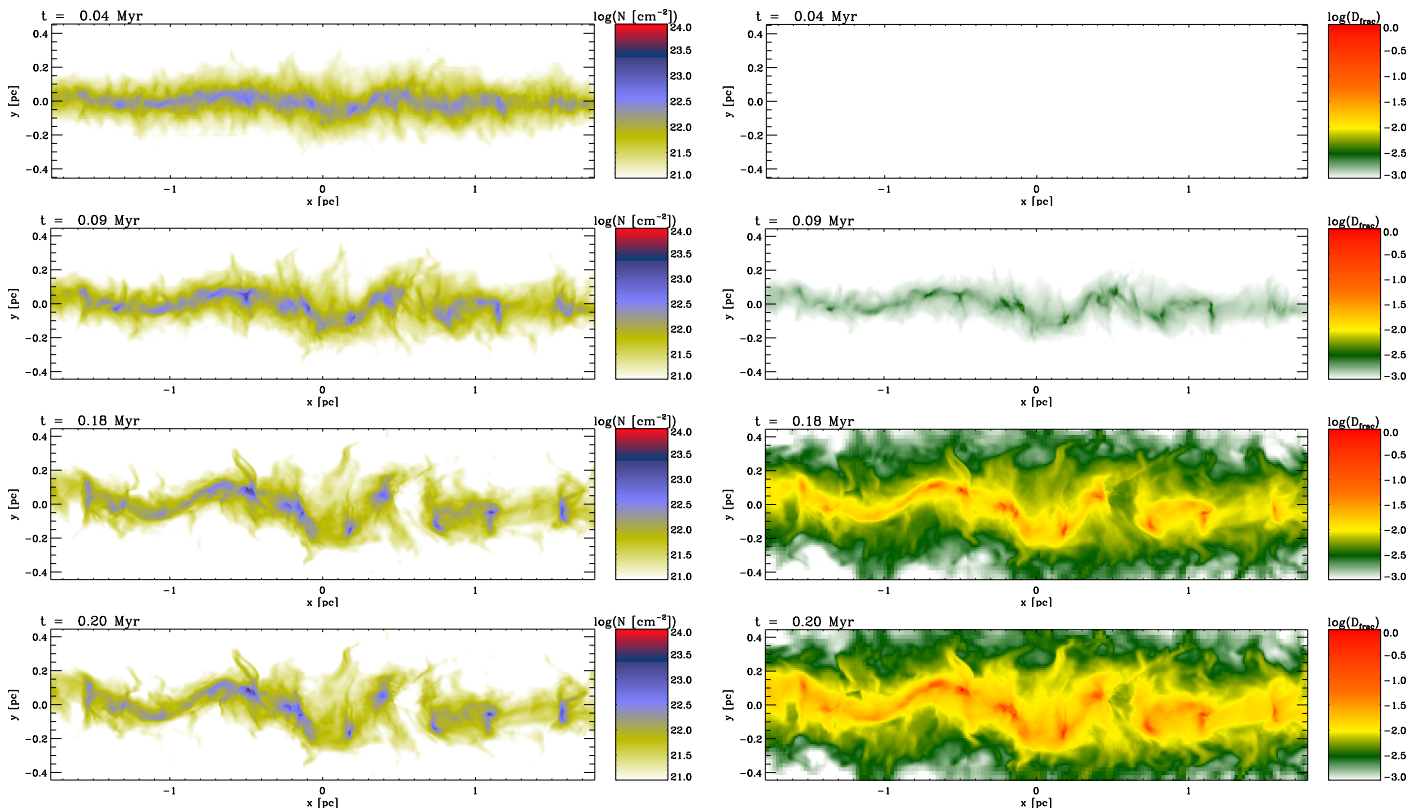
Figure 1. Time evolution of the filament in run ML1.6-M4.0-Para. Left: Top-down view of column density for the filament. Right: Same view for density-weighted deuteration fraction. The initially strong turbulence leads to a heavily bent and partially disrupted filament. Individual cores form due to compression. The times shown refer to 0.5, 1, 2, and 2.2 free-fall times. The integration length is l = 0.2 pc.
