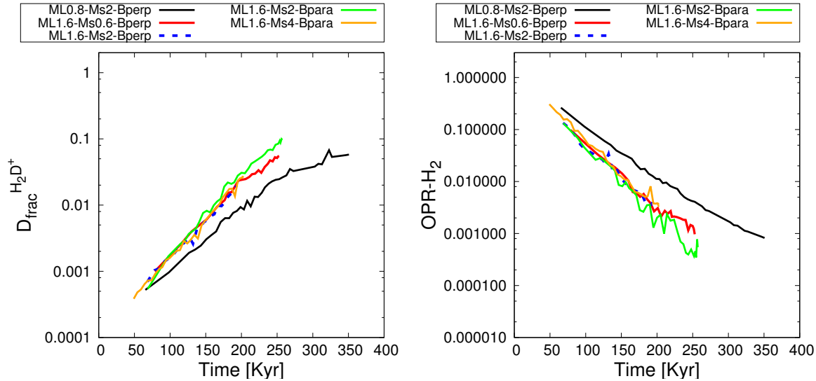
Figure 5. Time evolution of average deuteration fraction (left) and OPR-H 2 (right) in the cores given in Table 2. Although the initial OPR-H 2 is set to the conservative value of 3, the actual OPR at core formation is about an order of magnitude lower already after only 50 kyr ( \sim 0.5 t_{\text{ff,cyl}} ) of evolution.
