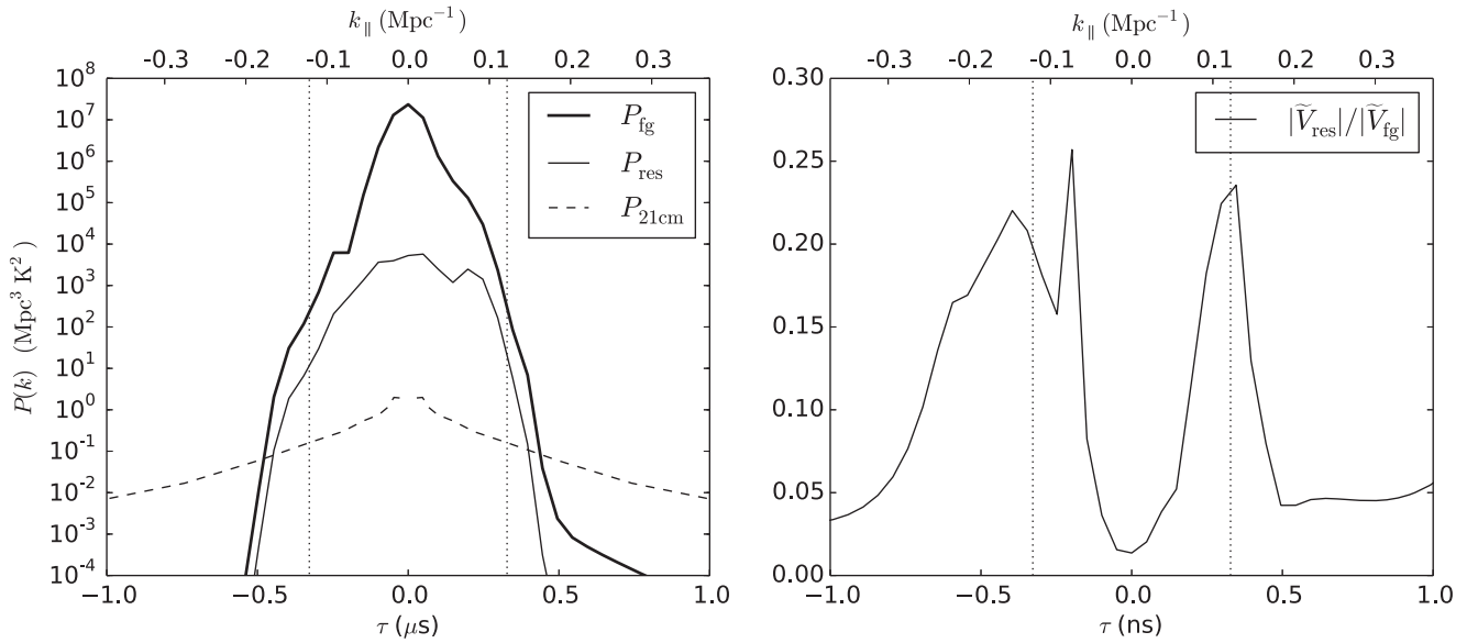
Figure 13. We simulate delay power spectra for a single baseline at 150 MHz ( z \sim 8.5 ) using the Global Sky Model and point source catalogs with and without beam-forming errors (dipole gain and delay errors of rms 0.5 dB and 50 ps and delay slope errors of rms 5 ps/MHz). We use a bandwidth of 20 MHz and a Blackman–Harris window function. Left: the total foreground power P_{\text{fg}} (thick black line) is predominantly contained within this baseline’s horizon limits (vertical dotted lines) where it dominates over the cosmological signal, but falls rapidly below that signal just outside the horizon limits (the “EOR window”). This demonstrates that the “foreground avoidance” approach reveals the cosmological signal even in the presence of frequency dependent beam-forming errors. Measurement of the cosmological signal within the baseline’s horizon limits, where it is largest, requires model subtraction with 3–4 orders of magnitude more dynamic range in power than is achieved by subtracting an otherwise perfect foreground model with unmodeled beam-forming errors P_{\text{res}} (thin black line). Right: the fractional visibility residual |V_{\text{res}}/V_{\text{fg}}| after subtraction is largest near the baseline’s horizon limits (corresponding to large zenith angles near the horizon, where the effects of beam-forming errors are largest, and lowest at zero delay (in the plane bisecting the baseline and including zenith).
