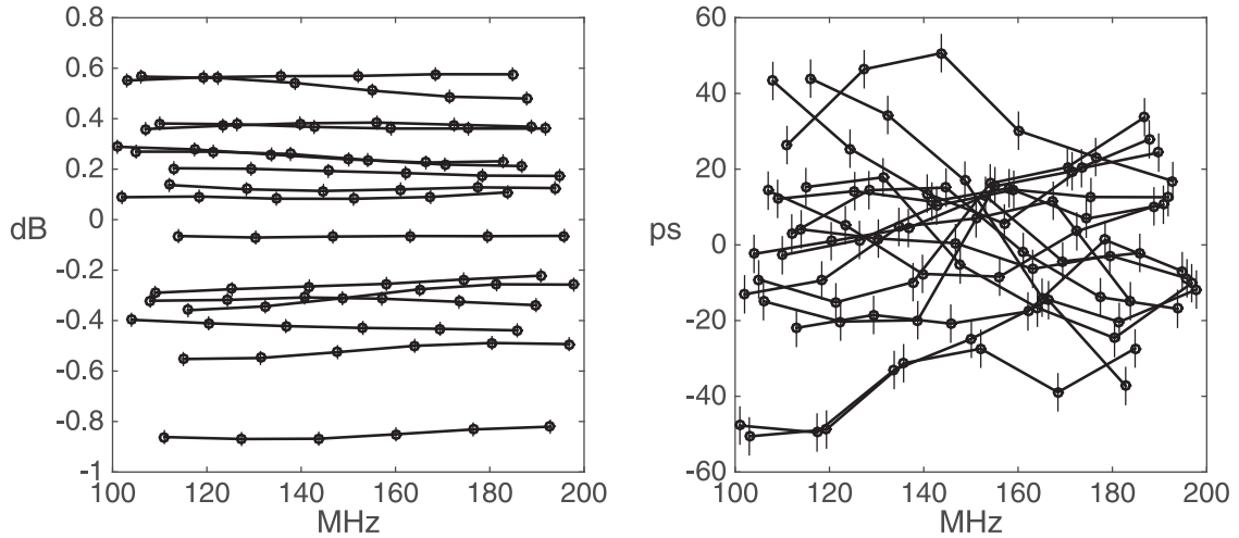
Figure 7. Gain and group delay measurements on the shortest delays of 16 beam-former inputs for one polarization are shown relative to the mean, as described in Section 2.2.3. Error bars of \pm 4.9 ps and \pm 0.026 dB are estimated from repeatability studies. At 150 MHz, an rms of 21 ps and 0.41 dB is observed. The worst cases are observed 2\sigma – 3\sigma away from the mean.
