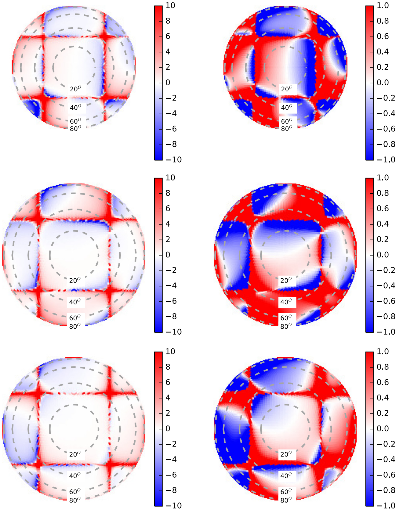
Figure 11. Each row shows a realization of a simulated beam error relative to the ideal beam (in dB) on a compressed color scale (left) and on an expanded color scale (right). This simulation used the full beam-forming error budget of \sigma_{\text{delay}} = 50 ps, \sigma_{\text{gain}} = 0.5 dB, \sigma_{\text{tilt,rot}} = 0.3^\circ . Here we see up and down fluctuations in the sidelobes and near the nulls (right) at the \pm 0.5 dB level seen in Figure 10, in addition to a positive bias within several degrees of the nulls (left).
