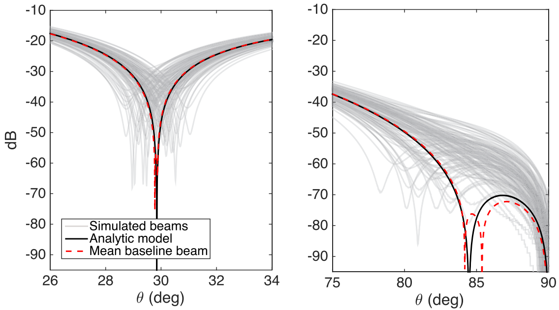
Figure 12. We zoom in around the first null and near the horizon along a NS slice through the beam after running simulations with our full beam-forming errors budget with 0^\circ 01 resolution. The nulls in all 128 beams with beam-forming errors ( |b_i|^2 ) (gray) are “filled in” by the errors; however, the baseline-averaged beam (Equation (3)) (red dashed) remains very close to the ideal power beam ( |b|^2 ) (black) for the reasons discussed in Section 3. This demonstrates that beam-forming fluctuations of different antennas tend to average out in imaging. Still, the antenna-to-antenna variation will limit deconvolution accuracy.
