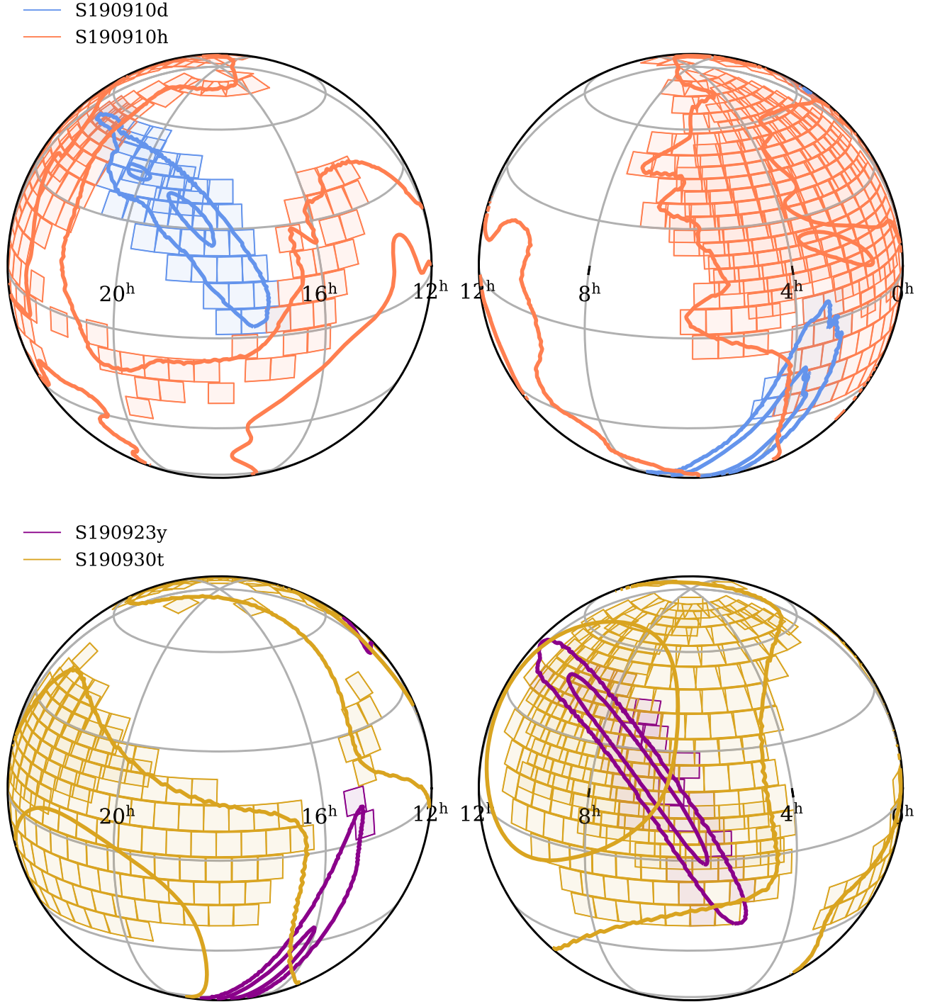
Figure 2. Top: ZTF coverage maps of the two same-day triggers occurring on September 10 (S190910d and S190910h) during O3 of LIGO/Virgo. Given the spatial and temporal overlap of these two GW triggers, some field observations contributed to coverage of both. Bottom: ZTF coverage maps of two NSBH triggers (S190923y and S190930t) during O3. Each square represents a ZTF pointing, and the solid line denotes the latest available GW 90% localization contour.
