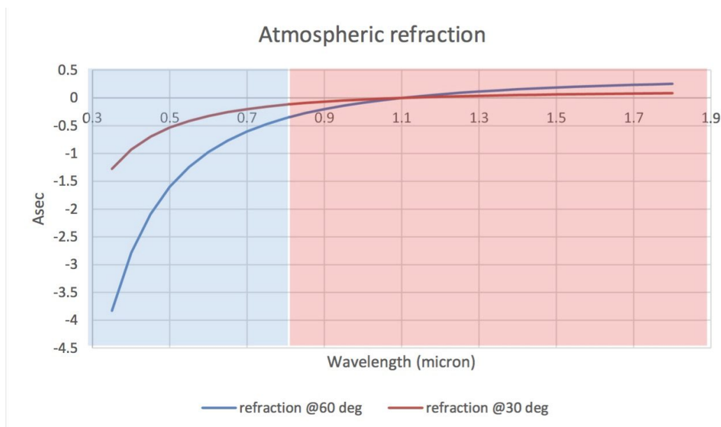
Figure 6. The trend of the atmospheric refraction in the visible (blue region) and in the NIR (red region) of the SOXS active wavelength range. The two curves are for different angles.
