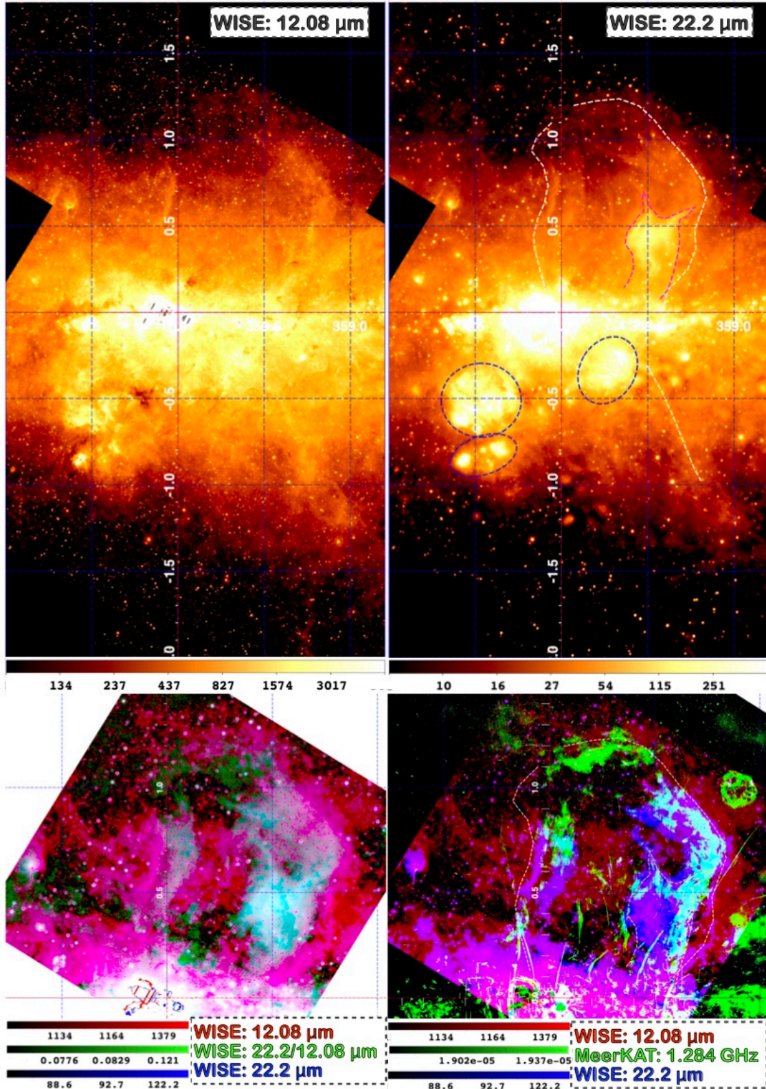
Fig. 6. Mid-IR emission from the central degrees of the Milky Way. ( Top left ) Emission at 12.08\ \mu\text{m} as observed by WISE . The highest concentration of warm dust is distributed along the Galactic plane. Spurs of material are clearly observed to emerge vertically from the plane. ( Top right ) Emission at 22.2\ \mu\text{m} as observed by WISE . The most prominent spurs of matter are highlighted by white dashed lines. At northern latitudes both the western and eastern spurs are clearly associated with the northern chimney and delineate a lobe clearly associated with the observed radio emission. The magenta dashed line delineates the silhouette of AFGL 5376. The detection of similar spurs in the southern hemisphere is complicated by the presence of well-known, bright foreground star-forming regions (highlighted by the blue ellipses). ( Bottom left ) Zoom-in toward the northern chimney. Red, green, and blue show the 12.08\ \mu\text{m} , the ratio 22.2\ \mu\text{m}/12.08\ \mu\text{m} , and 22.2\ \mu\text{m} emission, respectively. Warm dust surrounds the entire chimney. Also, the 22.2\ \mu\text{m} emission peaks inside the location of the western shock and of the 12.08\ \mu\text{m} emission spur. AFGL 5376 lies inside the edge of the warm gas and traces a \sim 90\ \text{pc} long molecular shock. ( Bottom right ) Same as previous but substituting the ratio map with the radio emission observed by MeerKAT . The radio emission is very well correlated with the warm dust emission. In particular, the radio emission traces the perimeter of AFGL 5376 more tightly than the warm dust emission.
