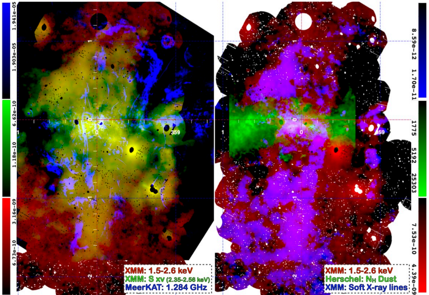
Fig. 5. Multiwavelength view of the chimneys. ( Left panel ) Red colors show the soft X-ray emission map (1.5-2.6 keV). Green colors show the S xv line emission (2.35-2.56 keV) and blue colors show the MeerKAT map. The S xv line emission shows clear gradients in rough coincidence with the edges of the MeerKAT bubbles. Additionally, it is less affected by interstellar absorption than the soft X-ray emission map (indeed the latter shows clear depressions in the emissivity of the chimneys at b \sim 0.2^\circ and b \sim -0.4 - 0.6^\circ ). ( Right panel ) RGB image of the GC. Red: Soft X-ray emission map (1.5-2.6 keV). Green: Column density map of neutral material as derived from dust emission of the central molecular zone, derived from Herschel observations (Molinari et al. 2011). The depressions of soft X-ray emission at b \sim 0.2^\circ and b \sim -0.4 - 0.6^\circ correspond to a high column density of neutral material, probably as a result of enhanced obscuration. We point out that the protrusion at l = 0.2, b = 0.25^\circ (§3.6) might be associated with a fountain originating from the Sgr B molecular complex, one of the most massive, highly obscured and highest star formation rate locations of the Milky Way. Indeed, although the protrusion appears to be disconnected from the plane in the soft X-ray map (it extends from b \sim 0.2^\circ to b \sim 0.6^\circ ), this might be a byproduct of strong obscuration in the Sgr B region. Blue: Continuum-subtracted soft X-ray line emission. The continuum subtraction removes the contribution from the dust-scattering haloes around bright point sources, which otherwise dominate the emission west of the southern chimney.
