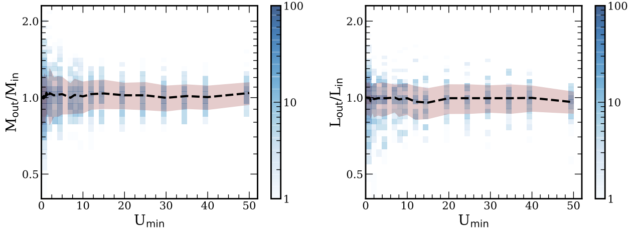
Fig. D.1. Simulations on the derivation of M_{dust} and L_{IR} . The ratio of derived over input M_{dust} (left) and L_{IR} (right) as a function of intrinsic \langle U_{min} \rangle for a range of simulated DL07 models mimicking the dynamical range and S/N of the available photometry for our stacked SEDs. For each U_{min} template the data are colour coded by the density of the points. The pink shaded region encloses the 68% of the derived ratios. Noticeably, the range of the output/input ratios, and thus the corresponding uncertainties are larger for colder templates ( U_{min} < 5.0 ).
