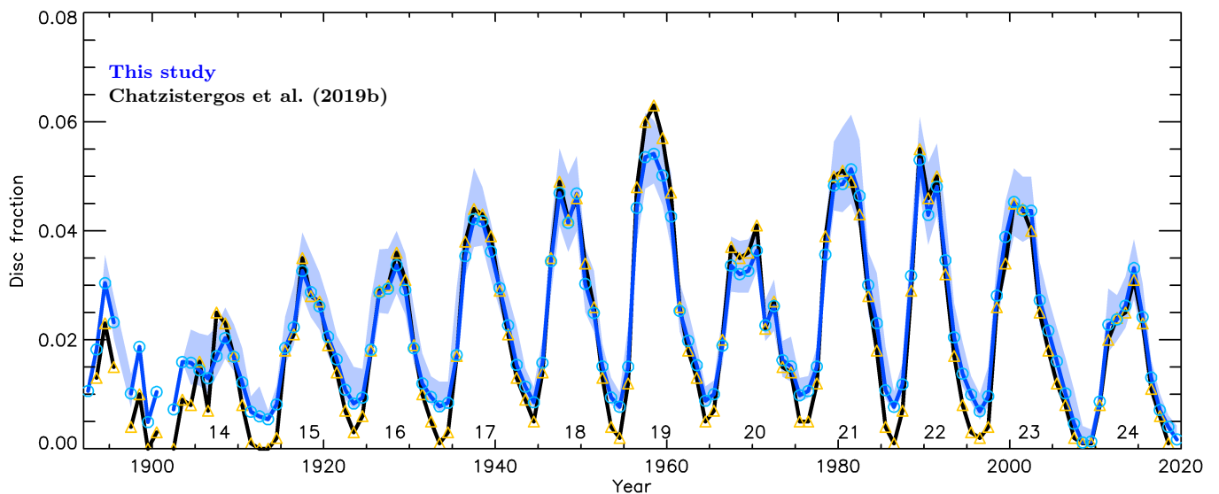
Fig. 9. Composite of plage areas in disc fraction derived in this study (blue line and blue circles) along with the composite by Chatzistergos et al. (2019b) (black line and yellow triangles). Shown are annual median values (solid lines and symbols) along with the asymmetric 1\sigma interval (shaded surfaces). The solar cycle numbers are given below the curves.
