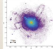
Fig. 1: stellar distribution at z=2.16 ( t_{\text{look}} = 10.5 Gyr)
