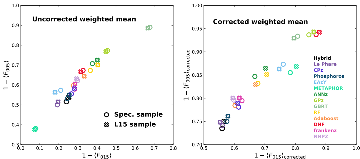
Fig. 9. PDZs metrics summarized by averaging the F_{005} and F_{015} values on all the bins with different weighting schemes. The axes are 1 - \langle F_{005} \rangle and 1 - \langle F_{015} \rangle to mimic the usual \sigma - \eta plots in Fig. 4. Left: results per bin weighted by the fraction of sources in the bin compared to the total number of sources kept by each methods (see Eq. (6)). Right: results of all the methods when correcting the \langle F_{005} \rangle and \langle F_{015} \rangle of each bin by the square root of the ratio of good sources in the bins to the number of sources that truly belong to the bin (see Eq. (7)). In each plot we include the results for the hybrid method (in black, see Sect. 5.4) for the weighted spectroscopic sample on the L15 sample.
