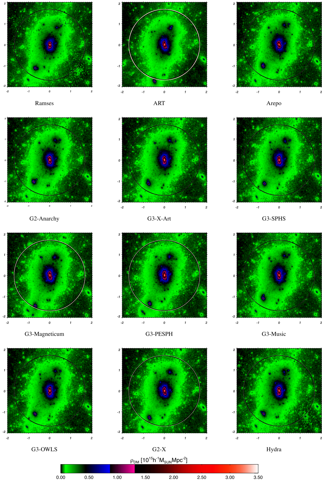
Figure 1. Projected density of the dark matter halo at z = 0 for each simulation as indicated. The box is 2 h^{-1} Mpc on a side. The white circle indicates M_{200}^{crit} for the halo, the black circle shows the same but for the G3-MUSIC simulation.
