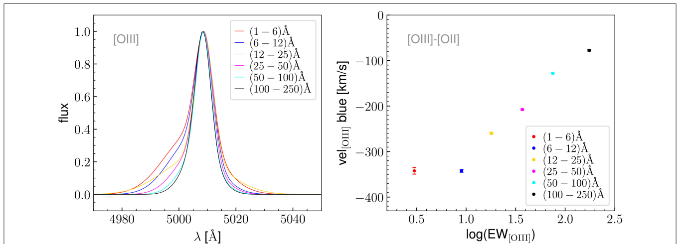
FIGURE 2 | Left: [OIII] 5007 Å line profile as a function of EW[OIII] . The blue component of the line decreases moving from low to high EW[OIII] . Right: velocity shift of the blue component of the [OIII] line with respect to the velocity of the [OII] \lambda 3727 line, accounting for the systemic velocity of the host galaxy. The shift is decreasing (in modulus) when moving from low to high EW[OIII] . Both the trends are expected if we are moving from face-on to edge-on positions, where the outflow velocity component of the gas is not intercepted anymore by the line of sight.
