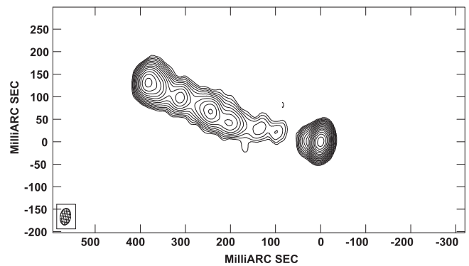
Figure 7. Highest-resolution ALMA image of 3C 138 at 241 GHz. The resolution is 37 \times 23 mas at P.A. = -11^\circ (shown by the cross-hatched ellipse). The contour levels are in multiplicative increments of \sqrt{2} . The peak flux is 0.095 \text{ Jy beam}^{-1} and the lowest contour is 0.33% of the peak.
