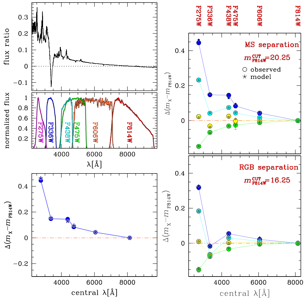
Figure 12. Left panels: the flux ratio between the best-fit comparison spectra of population E and population B for MS stars at m_{F814W}^{\text{CUT}} = 20.25 is plotted as a function of the wavelength in the upper panel, where we also show the normalized transmission curves of the filters used in this paper. Observed \Delta(m_X - m_{F814W}) against the central wavelength of the filter X are plotted with blue circles in the bottom-left panel. Asterisks are inferred from the best-fit synthetic spectra. Right panels: reproduction of Figure 10 where we plotted \Delta(m_X - m_{F814W}) as a function of the central wavelength of filter X as observed at m_{F814W}^{\text{CUT}} = 20.25 (top) and m_{F814W}^{\text{CUT}} = 16.25 (bottom). In addition, we show the synthetic colors corresponding to the best-fit model (see text for details).
