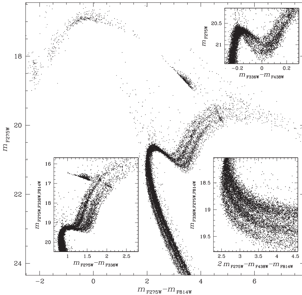
Figure 1. m_{F275W} vs. m_{F275W} - m_{F814W} CMD of NGC 2808. The m_{F275W,F336W,F814W} against m_{F275W} - m_{F336W} (bottom-left inset), m_{F336W,F275W,F814W} against 2 m_{F275W} - m_{F438W} - m_{F814W} (bottom-right inset), and m_{F275W} vs. m_{F336W} - m_{F438W} (upper-right inset) diagrams highlight multiple sequences along the RGB, the MS, and the SGB, respectively.
