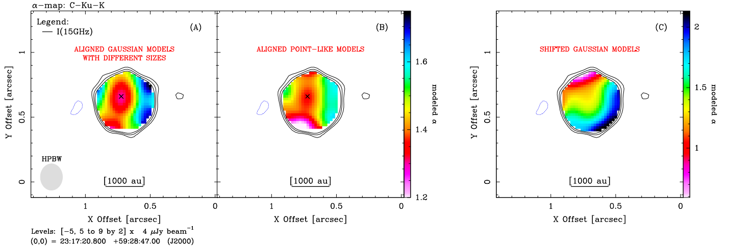
Fig. A.1. Simulated spectral index maps for field G111.24–1.24 in Fig. A.2. Labels and symbols as in Fig. 1. Panels a–c : spectral index maps (colors) obtained assuming three different source models at the C , Ku , and K bands. Black contours are those of the observed average brightness map for a direct comparison with Fig. A.2. The cross in panels a and b indicate the peak position of the observed C -band emission.
