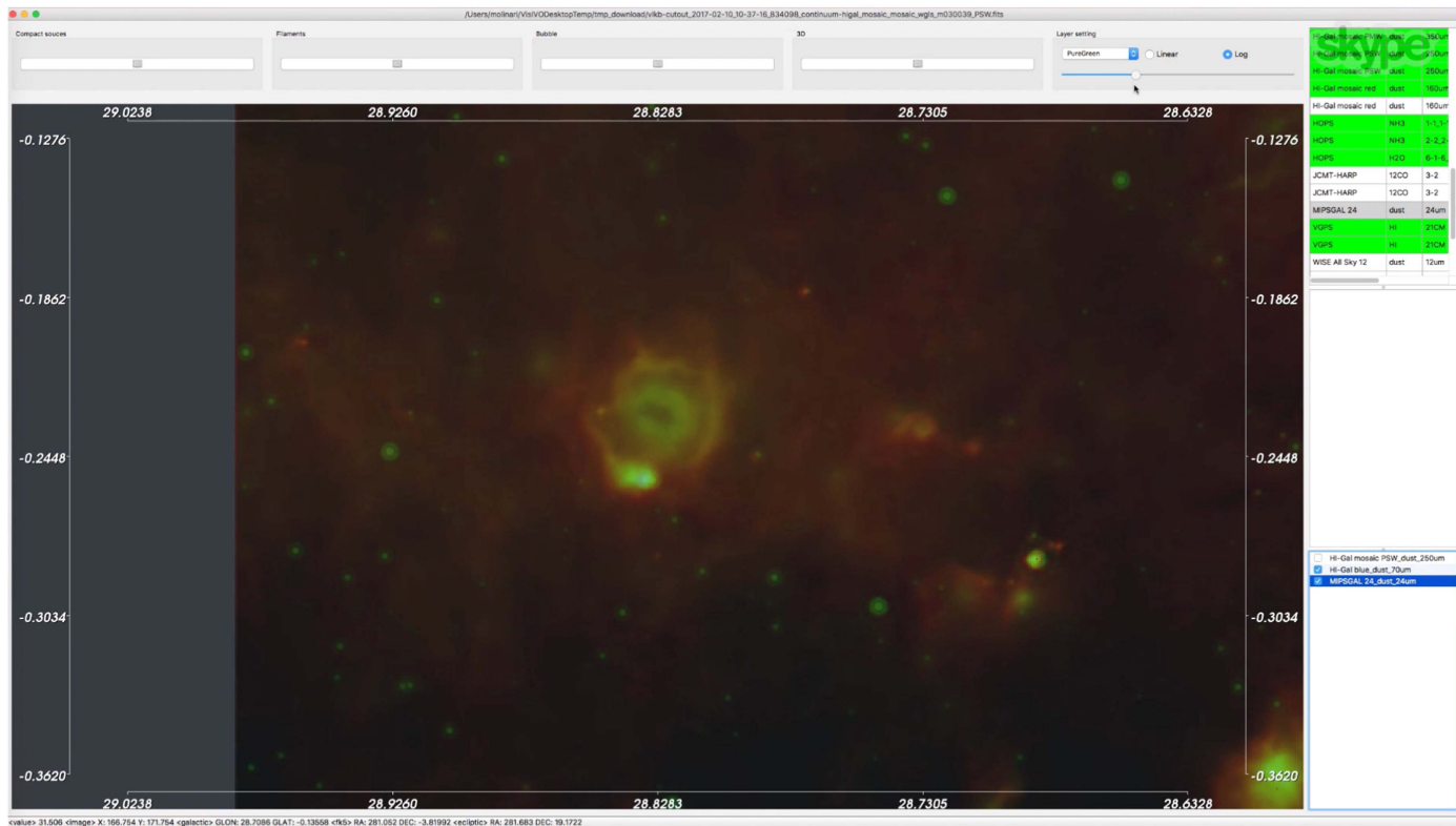
Figure 5. Bubble-like structure visualization. An Hi-GAL map at 70\ \mu\text{m} (with glow palette) superimposed on a 24\ \mu\text{m} MIPS GAL image (with pure green palette). (A color version of this figure is available in the online journal.)
