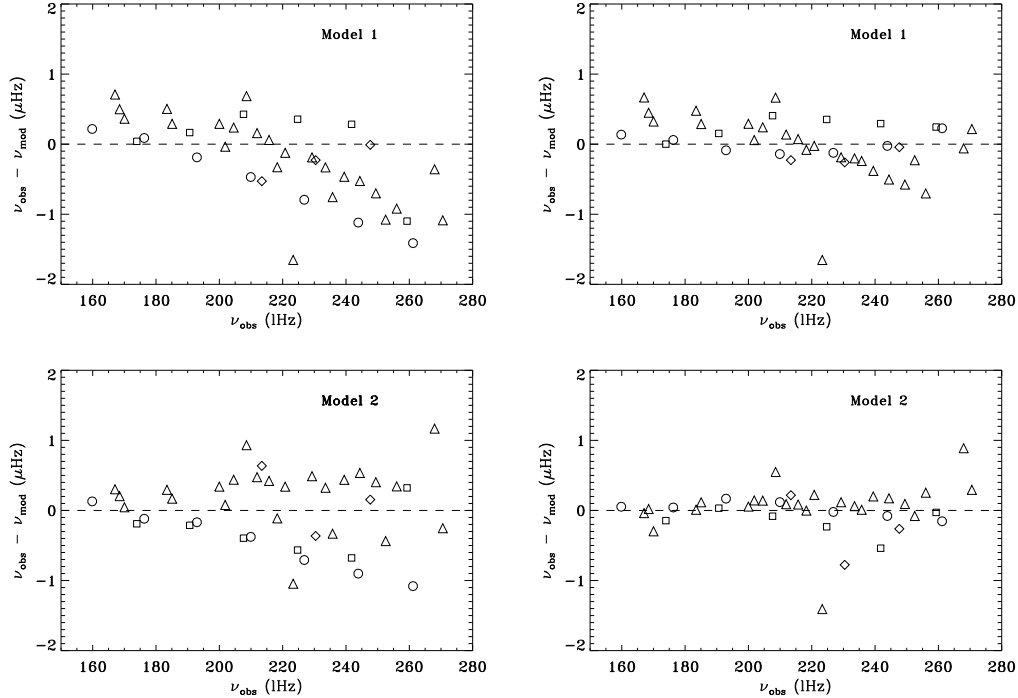
Figure 2. Differences between modelled and observed frequencies plotted against observed frequencies for Model 1 (upper row) and Model 2 (lower row) without correction (panels on the left) and with surface corrections (panels on the right). Circles are used for modes with l = 0 , triangles for l = 1 , squares for l = 2 , diamonds for l = 3 .
