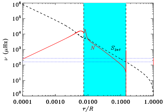
Figure 4. Propagation diagram for Model 2. The red solid-line represents the Buoyancy frequency, while the dashed line indicates the Lamb frequency for l = 1 . The blue dotted lines indicate the range of observed frequencies for KIC 4448777. The H-burning shell is shaded in light blue
