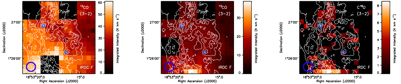
Fig. 4. Total integrated intensities for all detected components of the ^{12}\text{CO} ( left ), ^{13}\text{CO} ( centre ), and \text{C}^{18}\text{O} ( right ) J = 3 \rightarrow 2 lines towards IRDC F by the JCMT (in color scale). The contours give the mass surface density derived by Butler & Tan (2012) and are the same as in Fig. 1. The blue diamonds give the central locations of the F1 and F2 cores (right and left in the subfigures, respectively). The blue circle shows the HPBW of the observations.
