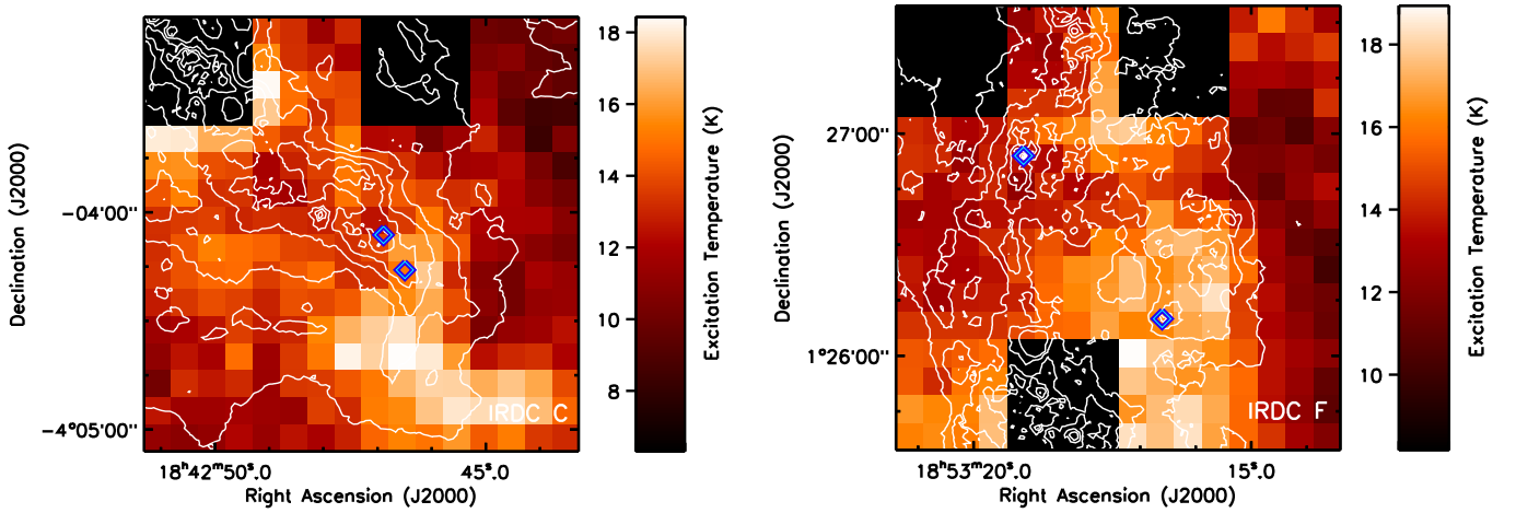
Fig. 6. Excitation temperatures based on the 12 CO J = 3 \rightarrow 2 line towards IRDC C ( left ) and IRDC F ( right ). The contours give the mass surface density derived by Butler & Tan (2012) and are the same as in Fig. 1. The blue diamonds give the central locations of the C1-N, C1-S, F1, and F2 cores.
