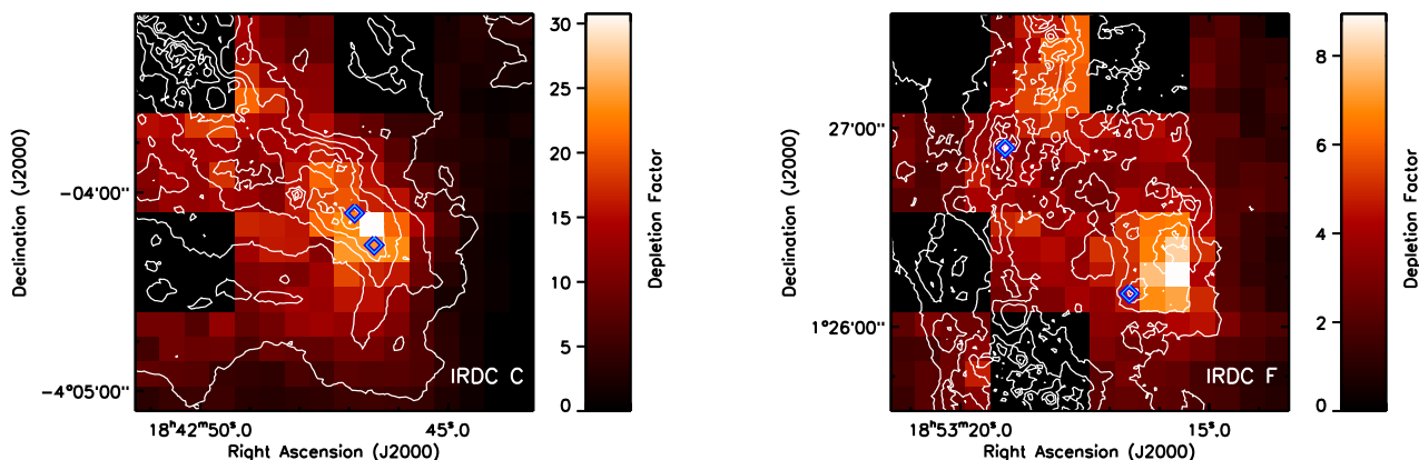
Fig. 8. CO depletion factor towards IRDC C ( left ) and IRDC F ( right ) derived under the assumption that the kinetic temperature for the ^{13}\text{CO} is the same as the ^{12}\text{CO} . The contours give the mass surface density derived by Butler & Tan (2012) and are the same as in Fig. 1. The blue diamonds give the central locations of the C1-N, C1-S, F1, and F2 cores.
