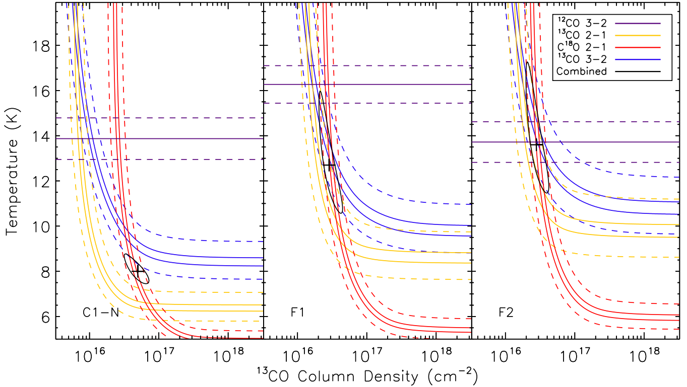
Fig. 7. Best fitting gas kinetic temperature and ^{13}\text{CO} column density ranges for the observed integrated intensities towards C1-N (left), F1 (centre), and F2 (right) based on RADEX modelling. The solid yellow, red, and blue lines show the models where the integrated intensities of the ^{13}\text{CO} J = 2 \rightarrow 1 , \text{C}^{18}\text{O} J = 2 \rightarrow 1 , and ^{13}\text{CO} J = 3 \rightarrow 2 , respectively, were within 5% of the observed values. The dashed yellow, red, and blue lines show the models where the models were within 25% of the observed intensities of the above three lines individually. The solid black ellipse shows the 1-sigma uncertainty range for models that match all three lines, found by the locus of models with a \chi^2 value within 1 of the best fitting model. The black cross indicates the best fitting model. The solid horizontal purple line gives the ^{12}\text{CO} J = 3 \rightarrow 2 derived temperature while the dashed purple lines give the uncertainty on this temperature.
