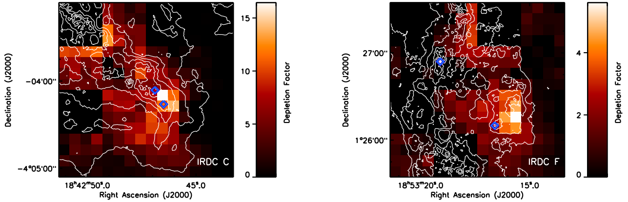
Fig. 9. CO depletion factor towards IRDC C (left) and IRDC F (right) derived under the assumption that the kinetic temperature for the ^{13}\text{CO} is 4 K less than for the ^{12}\text{CO} . The contours give the mass surface density derived by Butler & Tan (2012) and are the same as in Fig. 1. The blue diamonds give the central locations of the C1-N, C1-S, F1, and F2 cores.
