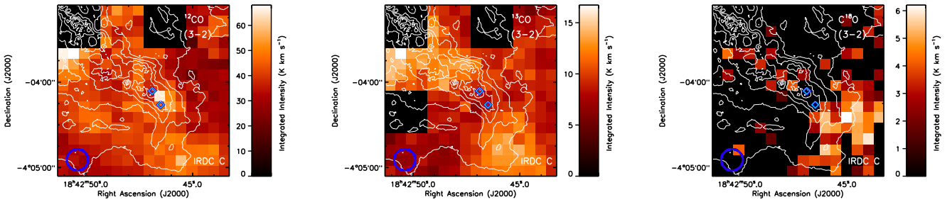
Fig. 3. Total integrated intensities for all detected components of the ^{12}\text{CO} ( left ), ^{13}\text{CO} ( centre ), and \text{C}^{18}\text{O} ( right ) J = 3 \rightarrow 2 lines towards IRDC C by the JCMT (in color scale). The contours give the mass surface density derived by Butler & Tan (2012) and are the same as in Fig. 1. The blue diamonds give the central locations of the C1-N and C1-S cores with the top left core in the subfigures being C1-N. The blue circle shows the HPBW of the observations.
