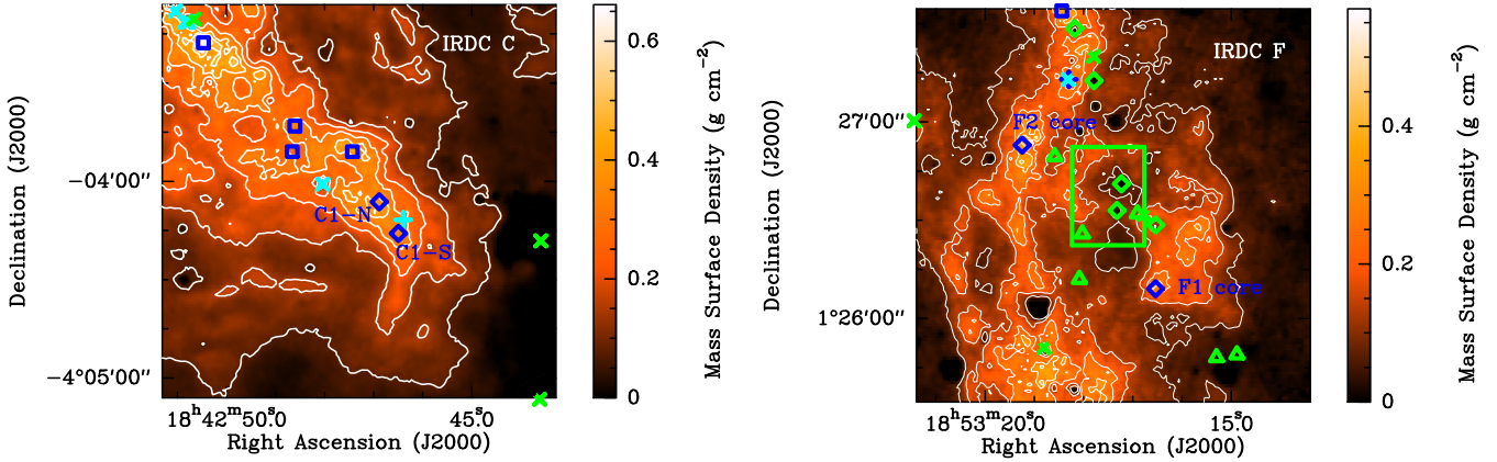
Fig. 1. Mass surface density derived by Butler & Tan (2012) for the C1 clump ( left ) and F1 and F2 clumps ( right ). The contours start at 0.075 \text{ g cm}^{-2} ( A_V of 17 mag) and increase by increments of 0.075 \text{ g cm}^{-2} with the typical uncertainty being of the order of 30% based upon uncertainties in the opacity per unit mass (Butler & Tan 2009, 2012). The uncertainty based upon background fluctuations is of the order of 0.013 \text{ g cm}^{-2} (Butler & Tan 2012). The dark blue diamonds give the central locations of the C1-N, C1-S, F1, and F2 cores, as determined from the \text{N}_2\text{D}^+ ALMA observations of Tan et al. (2013). The dark blue squares give the locations of extinction cores identified by Butler et al. (2014). The central location of the Butler et al. (2014) C1 clump is not shown in lieu of the Tan et al. (2013) locations. The light blue X's indicate the positions of water masers (Wang et al. 2006, 2012; Chambers et al. 2009) while the light blue cross indicates the position of the water maser detected at 59 \text{ km s}^{-1} by Wang et al. (2006) but not detected by the more sensitive survey of Chambers et al. (2009). The green X's indicate the positions of 70 \mu\text{m} sources from the HiGAL survey (Molinari et al. 2010). The green diamonds indicate positions of objects that were well fitted as young stellar objects (YSOs) by Shepherd et al. (2007). The green triangles are 24 \mu\text{m} sources that are likely YSOs, but which could also be asymptotic giant branch stars since they are only detected in two or less of the IRAC+2MASS bands (Shepherd et al. 2007). The green rectangle indicates the location of a near-infrared source overdensity (overdensity A), interpreted by Foster et al. (2014) as an embedded low mass protostar population. The right ascension for this overdensity given in Table 3 of Foster et al. (2014) is incorrect (Foster, pers. comm.) and we use a right ascension of 18^{\text{h}}53^{\text{m}}17^{\text{s}} (J2000), not 8^{\text{h}}53^{\text{m}}20^{\text{s}} (J2000), for this overdensity. The regions shown are the regions mapped by the JCMT.
