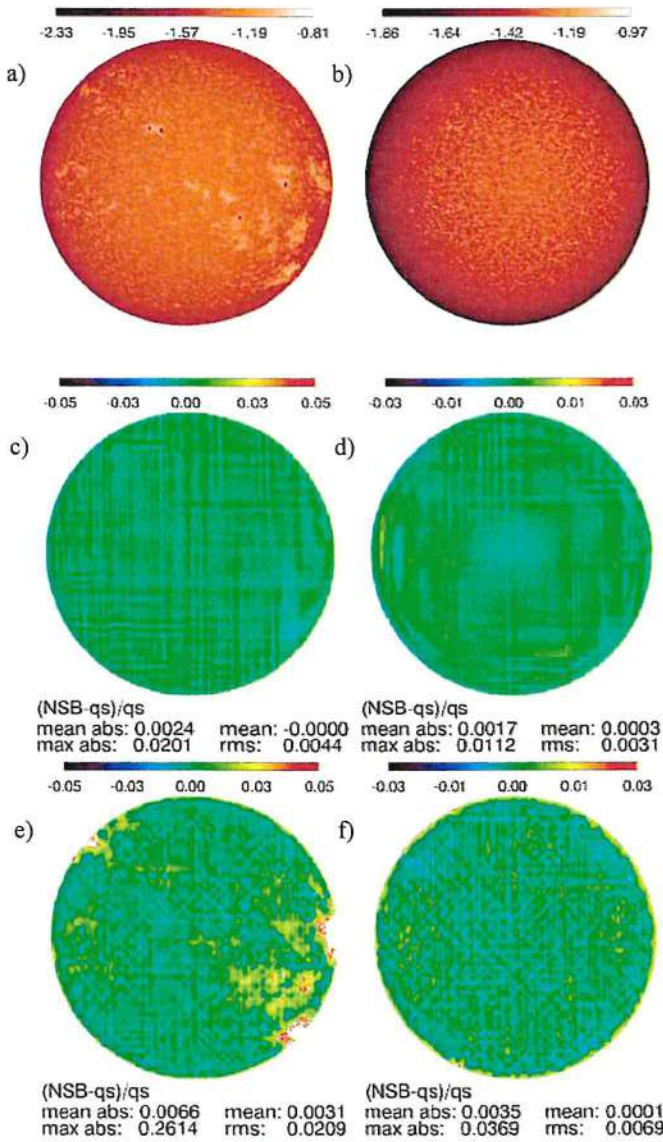
Fig. 15. Relative error in NSB calculation with our method ( c–d ) and the method by Worden et al. (1998a, e–f ) for two images of subset 6 with the lowest level of inhomogeneities (density images shown on a–b ). The facular pattern was derived from the Rome/PSPT observations taken on 21/08/2000 ( left ) and 09/08/2008 ( right ). Also given (below the images) are the values of the rms, mean, mean absolute and maximum relative differences within the disc up to 0.98 R . The colour bars apply to the images below them.
