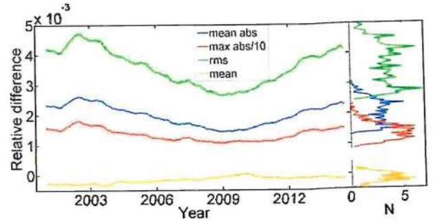
Fig. A.2. Left: relative difference between the NSB and the imposed background for all images of subset 1 (disc positions within 0.98 R ). For clarity, the maximum difference is divided by ten. The solid lines are 30 point averages and the shaded surfaces denote the asymmetric 1\sigma intervals. Right: distribution functions of the difference values.
