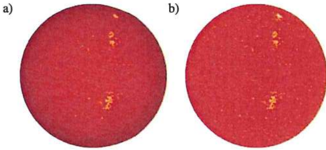
Fig. 5. Panel a: photometrically calibrated, and panel b: contrast image corrected for the CLV for the Ko observation shown in Fig. 3. The colour scale of the calibrated image covers the full range of intensities on the disc, while the contrast image is shown within the intensity range [-1, 1] .
