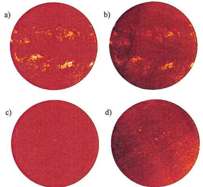
Fig. 17. Examples of calibrated and CLV compensated images from the Ko archive derived with our method ( left ) and with the method of Priyal et al. (2013, right ); the latter data were taken from the Kodaikanal website. The results from Priyal et al. (2013, right ) are given in JPG files and shown here unsaturated, while the results from our processing are saturated in the range [-0.5, 0.6] . The observations were taken on 05/08/1947 ( top ) and 01/01/1964 ( bottom ).
