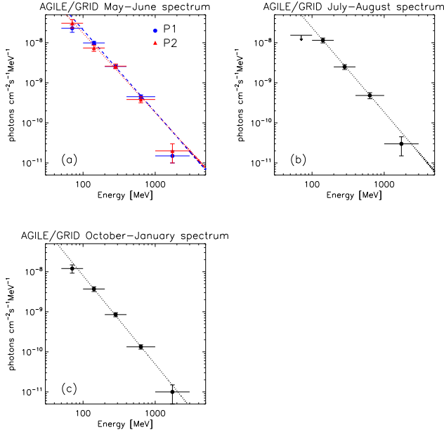
FIG. 2.— Panel (a): AGILE/GRID average \gamma -ray spectrum for periods P1 and P2. The blue-dashed and the red-dotted lines represent the best-fit power law models for P1 and P2, respectively. Panel (b) and Panel (c) show the average \gamma -ray spectra during the periods July–August 2008 and October 2008 - January 2009, respectively. In the three panels only three energy bins were considered for the spectral fitting: 100 < E < 200 MeV, 200 < E < 400 MeV, 400 < E < 1000 MeV (see text for details). [See the electronic edition of the Journal for a color version of this figure.]
