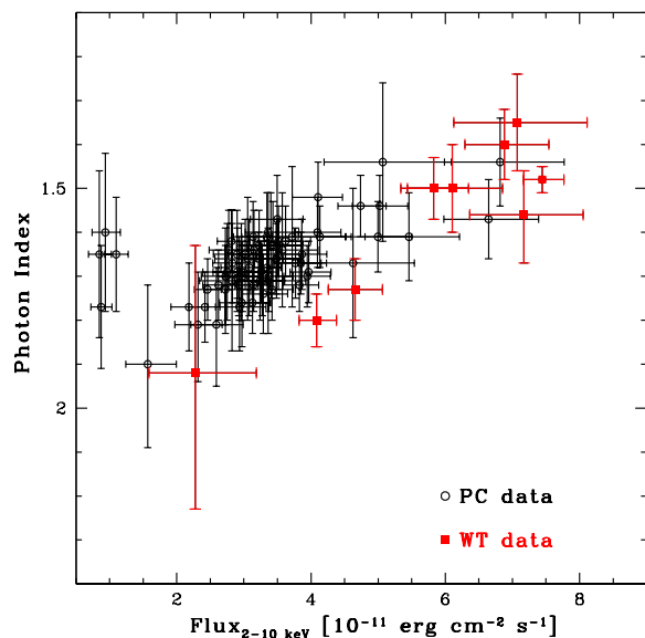
FIG. 4.— Swift /XRT photon index as a function of the 2–10 keV flux. Red squares and black circles mark the Swift /XRT windowed timing (WT) and photon counting (PC) data, respectively.
