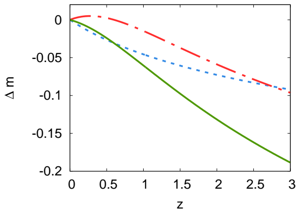
FIG. 4. Differential effects on the apparent magnitude of a standard candle induced by the torsion model given in (82) in comparison to a reference \Lambda CDM model. Top curve (dot-dashed red): 5 \log_{10} \Delta_D ; middle curve (dotted blue): 5 \log_{10}(1 + \eta) ; bottom curve (solid green): 5 \log_{10}(1 + \eta) + 5 \log_{10} \Delta_D . The bottom line shows the total change of magnitude within the approximation of weak torsion and with \eta_0 = -0.03 . As seen a change of magnitude of order of \Delta m = 0.1 is small (compared to for example the scatter of supernovae data) but still it is not negligibly small, and could be mistaken (for example) for the evolution of sources, with sources misinterpreted to be brighter at larger redshift.
