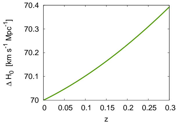
FIG. 5. The impact of cosmological torsion on the inferred value of H_0 as a function of redshift of the data used, i.e. if one uses data at z \approx 0.3 , then the inferred value of H_0 is greater by 0.4 \text{ km s}^{-1} \text{ Mpc}^{-1} compared to H_0 inferred from the data at z \approx 0 . The effect of torsion on the luminosity distance was evaluated within the approximation of weak torsion, i.e. (77) with (82) and \eta_0 = -0.03 .
