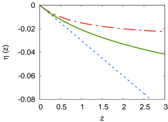
FIG. 3. The deviation \eta (63) of the distance duality relation evaluated in the limit of weak torsion (77), as a function of redshift z for three different torsion models with \eta_0 = -0.03 . Bottom curve (dotted blue) (78); middle curve (solid green) (79); top curve (dot-dashed red): (81).
