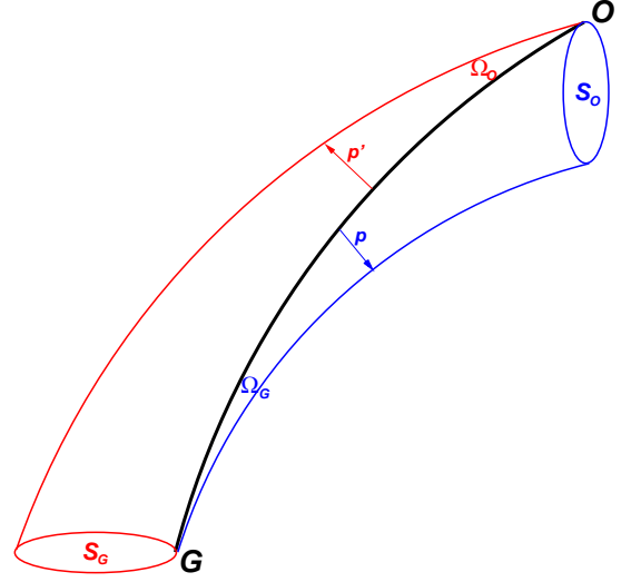
FIG. 2. Deviation of light rays around the null curve GO linking an observed galaxy with the observer, after [15, Fig. 7], with several differences in notation. Quantities at the emission event (i.e. at G) are labelled with G, while quantities at the observation event (i.e. at O) are labelled with O. The connecting vector between the light curves that diverge towards the observer is p^\alpha and the cross section of the diverging bundle at the observation event is S_O (the observed flux and hence luminosity distance depends on S_O ). The connecting vector between the light curves that converge towards the observer is p'^\alpha and the rate of convergence is proportional to \Omega_O (the observed angular size and hence angular diameter distance depends on \Omega_O ).
