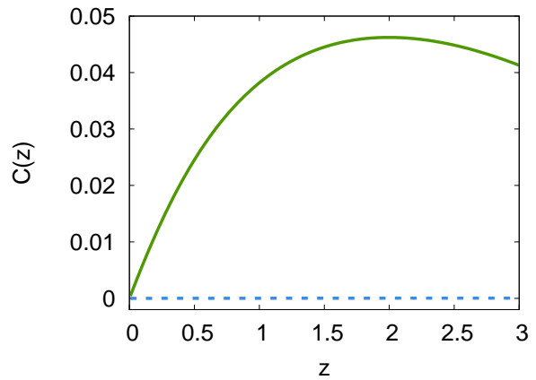
FIG. 6. The CBL parameter as given by eq. (86). If the distance D is obtained from the angular diameter distance (69), (70), then the CBL parameter is zero, \mathcal{C}(z) = 0 (flat blue curve). If the distance is inferred from supernovae type Ia distance modulus observations, i.e. from the luminosity distance (71), without accounting for the presence of torsion via the parameter \eta , then \mathcal{C}(z) \neq 0 (green curve). The torsion model here is the same as for the other figures (82), i.e. \phi = \eta_0 H , \eta_0 = -0.03 .
