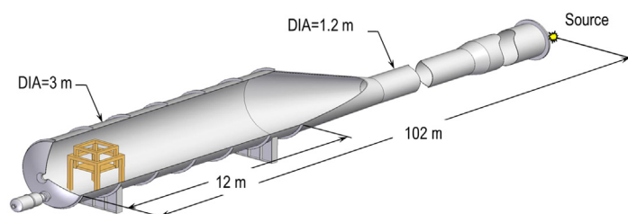
Fig. 7 The MSFC SLTF. The hexapod is shown in gold.
