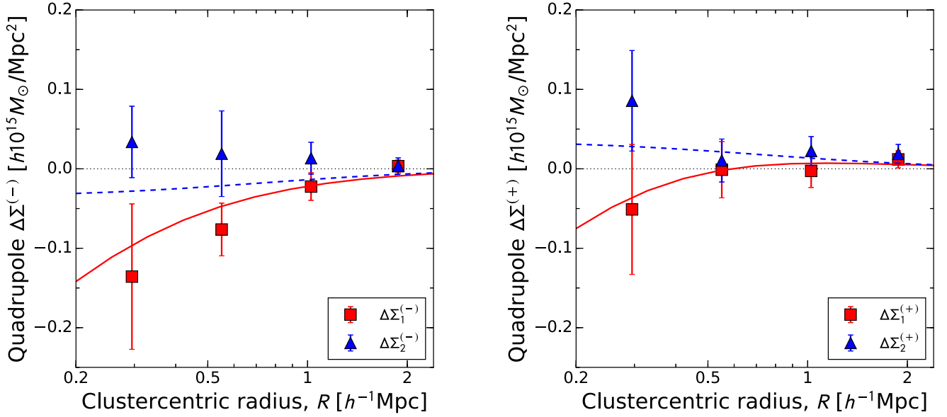
Figure 8. Stacked quadrupole shear profiles for our sample of 20 CLASH clusters measured with respect to the X-ray major axis of each cluster. Left panel: the observed \langle \Delta \Sigma_1^{(-)} \rangle (red squares) and \langle \Delta \Sigma_2^{(-)} \rangle (blue triangles) profiles shown along with the best-fit elliptical NFW (eNFW) model. Right panel: the same as the left panel, but showing the results for the \langle \Delta \Sigma_{1,2}^{(+)} \rangle profiles. The best-fit model was obtained from a simultaneous eNFW fit to the four quadrupole shear profiles.
