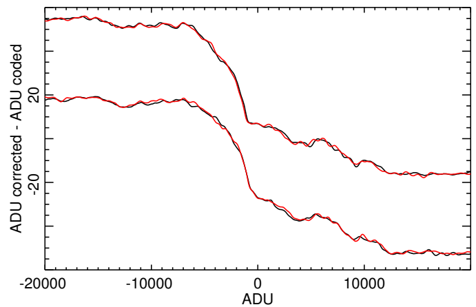
Figure 5. Example ADC correction functions for both parities (upper and lower curve sets) and two different phases (in black and red) relative to the 4 He-JT cooler cycle.
