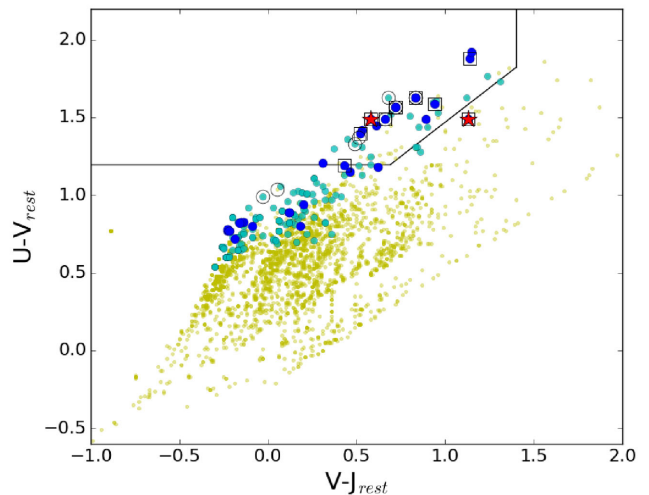
Figure 6. UVJ diagram for z_{\text{CANDELS}} > 3 sources, computed adopting the standard \tau -models to derive the rest-frame magnitudes. The passive selection region is defined by (U - V) > 0.88 \times (V - J) + 0.59 , (U - V) > 1.2 and (V - J) < 1.4 (Whitaker et al. 2011). Yellow points are the whole sample of z > 3 , Ks+3.6+4.5 \mu\text{m} H -detected galaxies from G13. Cyan small dots refer to the objects having a passive best-fitting model, both with and without the inclusion of the emission lines in the TH library. Blue large dots are the 30 galaxies in the reference sample, with empty squares indicating the 10 sources selected also including nebular emission lines. The red stars refer to the candidates surviving the z -free selection. Finally, empty circles refer to the \tau -model red and dead selection ( \text{sSFR} < 10^{-11} \text{ yr}^{-1} ; Section 5). Not all the galaxies in the selections are visible because some models have very similar rest-frame properties and colours, so that the symbols overlap. [A colour version of this figure is available in the online version.]
