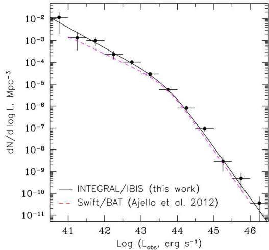
Figure 9: Observed hard X-ray luminosity function of local AGN (circles) fitted by a broken power law (solid line). For comparison, the luminosity function based on the Swift /BAT survey (Ajello et al., 2012) is shown by the dashed line. From (Sazonov et al., 2015).
