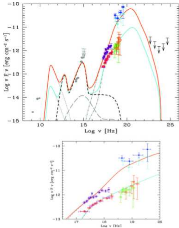
Figure 15: Top: spectral energy distribution of IGR J22517+2217. Grey circles and arrows represent archival radio/optical/UV data from NED. Red triangles and magenta squares represent XIS 0 and XIS 3 data, green circles and orange pentagons represent PIN and BAT quiescent data respectively, while black arrows are Fermi upper limits in five bands. Filled violet squares represent XRT data, filled cyan diamonds and blue pentagons represent IBIS and BAT flare data respectively. The solid cyan and orange curves are the results of modelling of the quiescent and flaring states, respectively. With grey lines we show the different components of non-thermal emission: synchrotron (dotted), synchrotron self-Compton (long-dashed) and external Compton (dot-dashed). The black dashed line corresponds to the thermal emission of the disc, the IR torus and the X-ray disc corona. The model does not account for radio emission, produced from much larger regions of the jet. Bottom: enlargement in the X-ray energy range for the two SEDs. Symbols as in the top panel. Figure from Lanzuisi et al. (2012)
