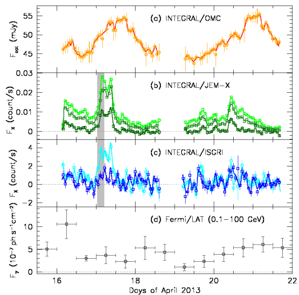
Figure 14: Light curve of MKN 421 in April 2013, see Pian et al. (2014)
