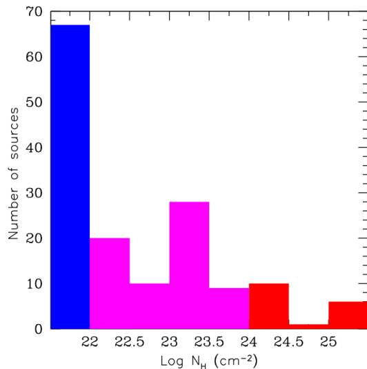
Figure 7: Observed distribution of absorption columns. Unabsorbed ( N_{\text{H}} < 10^{22} \text{ cm}^{-2} ), weakly absorbed ( 10^{22} \leq N_{\text{H}} \leq 10^{24} \text{ cm}^{-2} ) and Compton-thick ( N_{\text{H}} \geq 10^{24} \text{ cm}^{-2} ) objects are shown in blue, magenta and red, respectively. From (Sazonov et al., 2015).
