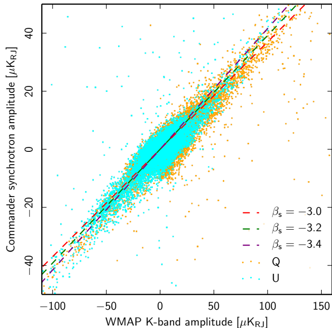
Fig. 48. T - T correlation plot between the Planck polarized synchrotron map at 30 GHz and the WMAP K -band map at 23 GHz for both Stokes Q and U parameters. The dashed coloured lines indicate synchrotron spectral indices of \beta_s = -3.0 (red), -3.2 (green) and -3.4 (violet), respectively.
