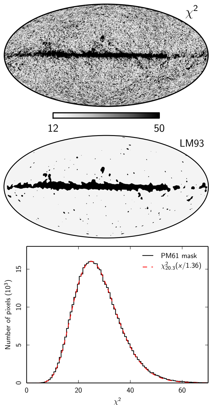
Fig. 22. Top: \chi^2 per pixel for joint baseline Planck , WMAP, and 408 MHz intensity analysis. Middle: confidence mask derived by smoothing the \chi^2 map to 1° FWHM, and thresholding at a value of \chi^2_{\max} = 50 . Its primary application is for the low- \ell 2015 Planck temperature likelihood, and it is accordingly denoted LM93 (93% likelihood mask); see Planck Collaboration XI (2016) for further details. Bottom: histogram of \chi^2 values outside the conservative PM61 mask. The grey dashed line shows the best-fit \chi^2 distribution with a variable degree of freedom and scaling, used to account for prior and noise modelling effects; see Sect. 5.3 for further discussion.
