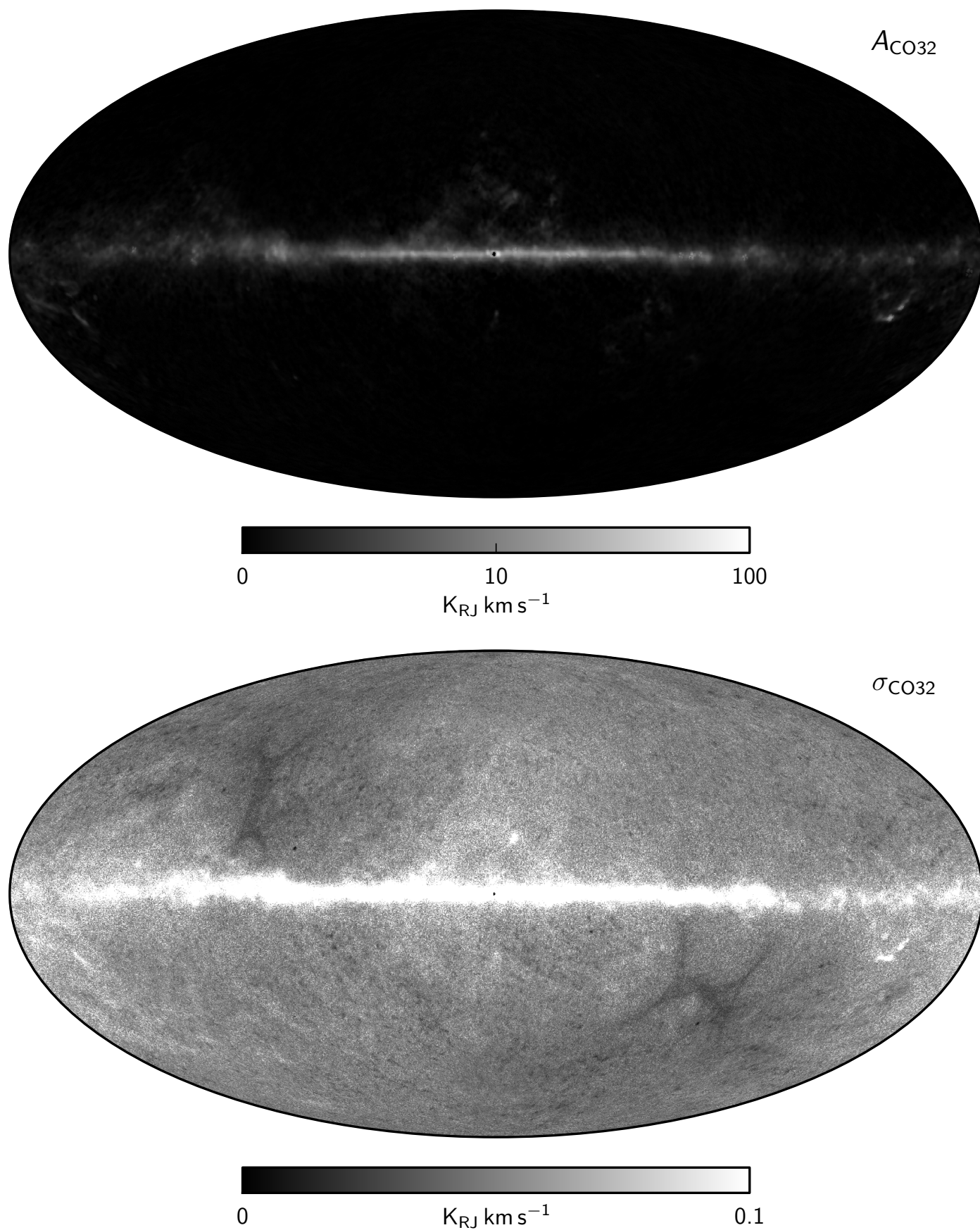
Fig. 15. Maximum posterior ( top ) and posterior rms ( bottom ) CO J=3 \rightarrow 2 line emission maps derived from the joint baseline analysis of Planck , WMAP, and 408 MHz observations. The top panel employs a non-linear high dynamic range colour scale, while the bottom panel employs a regular linear colour scale.
