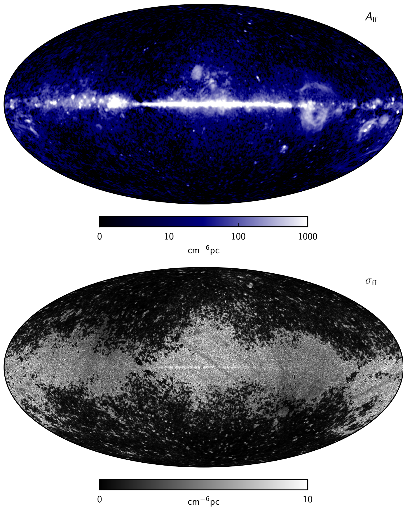
Fig. 9. Maximum posterior ( top ) and posterior rms ( bottom ) free-free emission measure maps derived from the joint baseline analysis of Planck , WMAP, and 408 MHz observations. The top panel employs a non-linear high dynamic range colour scale, while the bottom panel employs a regular linear colour scale.
