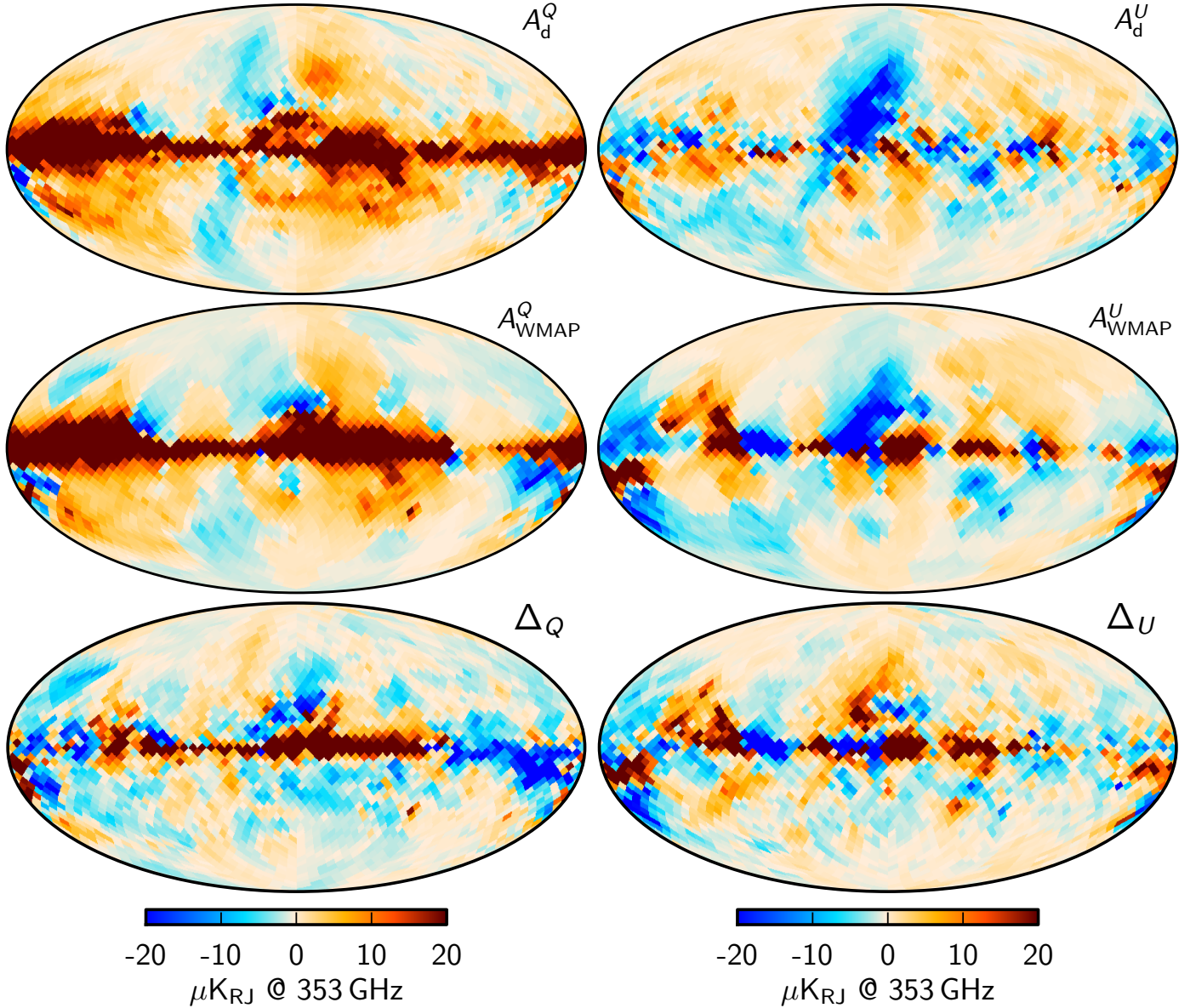
Fig. 47. Comparison of the Planck polarized thermal dust map at 353 GHz ( top ) and the WMAP polarized dust template, scaled to 353 GHz assuming a scaling factor of 480 \mu\text{K} ( middle ). The bottom row shows the difference between the two maps. All maps are pixelized at a HEALPix resolution of N_{\text{side}} = 16 .
