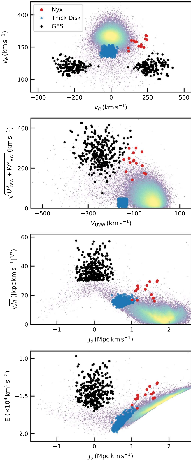
Figure 3. The orbital properties of the entire GALAH survey within 3 kpc of the Sun. Highlighted are the Nyx stars (red dots), Gaia-Enceladus stars (black dots), and a kinematic selection of thick disk stars (blue dots); the background distribution in each panel is a scatter log-density plot of all stars.
