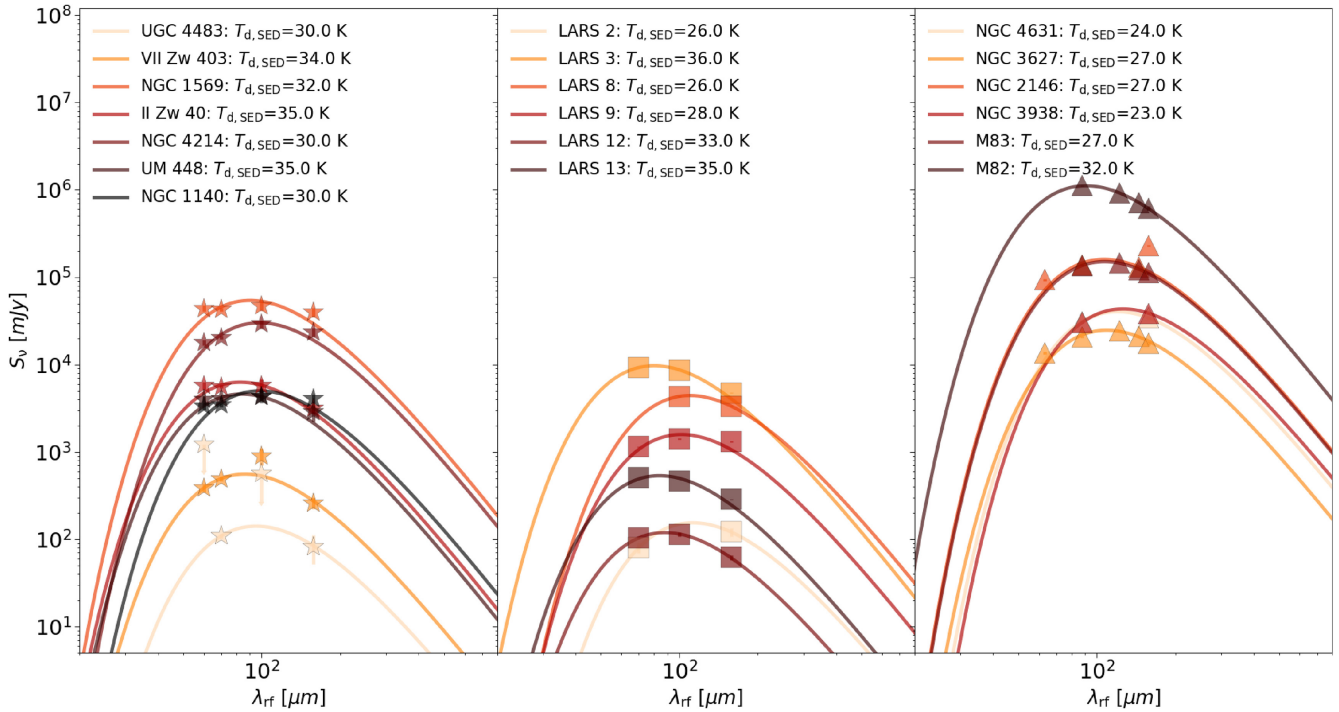
Figure B1. FIR SED grey-body fit ( \beta_{\text{d}} = 2.0 ) for the galaxies in the local sample. From left to right: DL subsample (Nilson 1973; Engelbracht et al. 2008; DL; Cormier et al. 2019, ID 0-6 in the paper), LARS subsample (Puschig et al. 2020, ID 7-12), and PACS data base subsample (Jarrett et al. 2003; Caldú-Primo & Cruz-González 2008; Leroy et al. 2008; Groves et al. 2015; Fernandez-Ontiveros et al. 2016, ID 13-18). In all cases, we find consistent temperatures (within the errors) with the ones obtained through continuum fluxes ratio in the paper (See Table 1).
