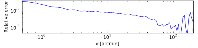
Fig. 12. Reduced shear effects: relative two-point correlation error between the mean two-point correlation functions \xi_+^{\mathcal{E}^{\gamma}} estimated from the shear fields and corresponding mean two-point correlation function \xi_+^{\mathcal{E}^g} estimated from the reduced shear fields without any correction.
