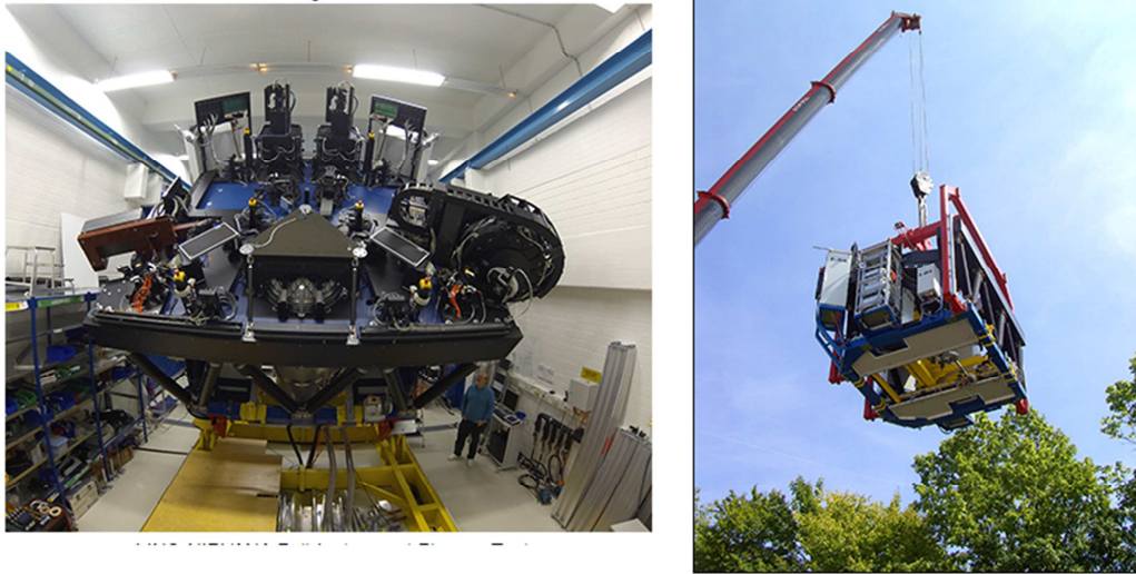
Fig 2: Left: Before PAE, “flexure-test” was performed. Right: “flight-test” before packing
