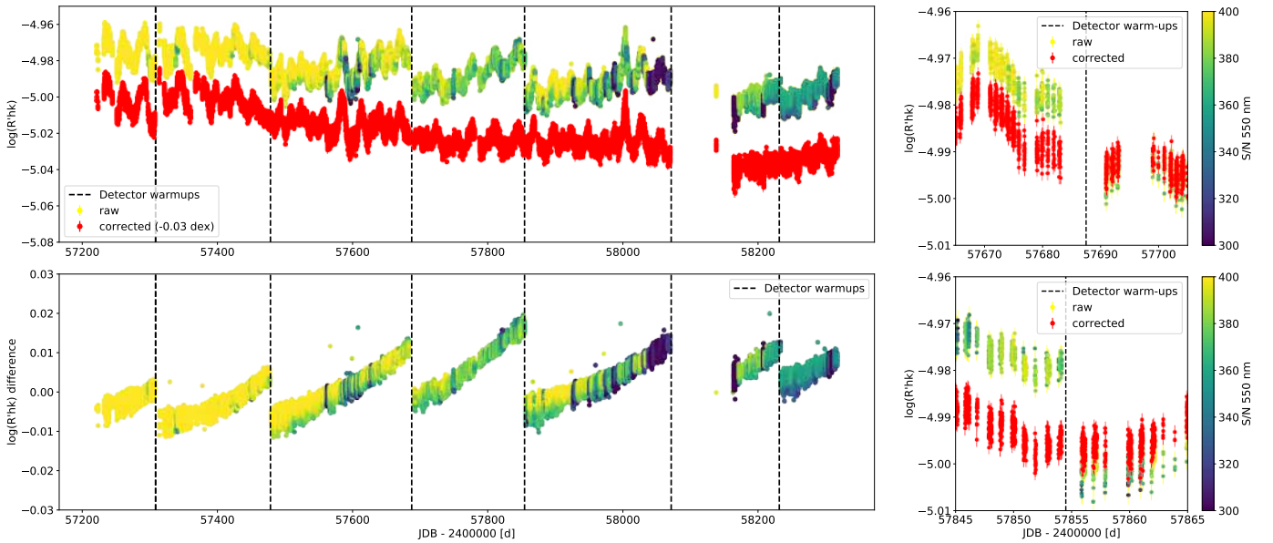
Fig. 6. Top left: comparison between the raw (dots with yellow to blue colour scale) and corrected (red dots) \log(R'_{\text{HK}}) calcium activity index, as described in the text. Bottom left: differences between the raw and corrected \log(R'_{\text{HK}}) time series. We clearly see that the slow increase in the activity index followed by sudden jumps at each warm-up of the detector seen in the raw \log(R'_{\text{HK}}) time series is strongly reduced after correction. Top and bottom right: closer look at the regions around the third and fourth warm-ups.
