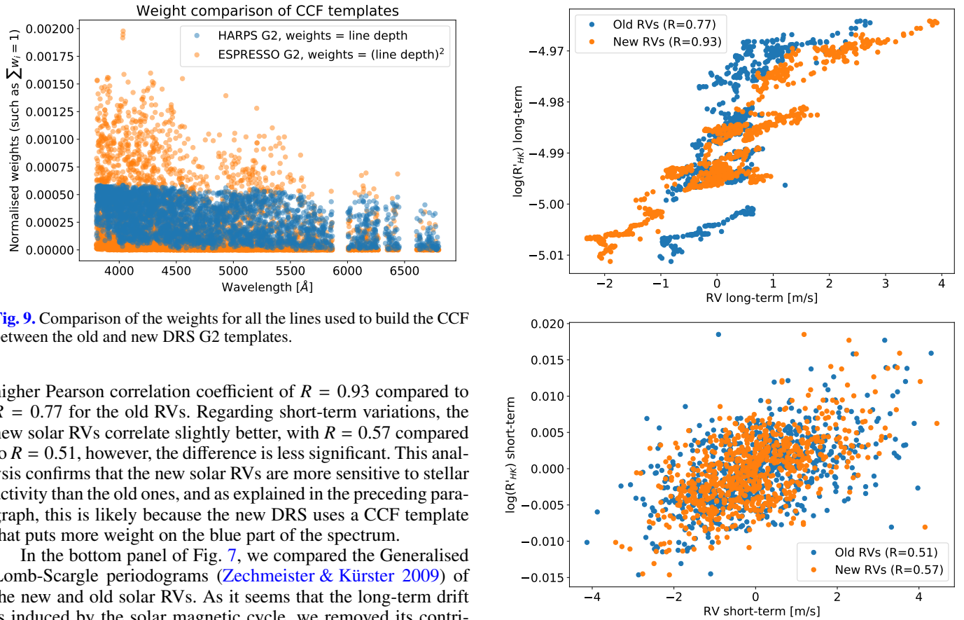
Fig. 10. Top: correlation between the RVs and the \log(R'_{\text{HK}}) for long-term variations, which in this case means that the time series were smoothed using a 30-day rolling average. Bottom: correlation between the short-term variations, meaning the raw time series minus the smoothed ones. In the legend, we show the values for the R Pearson correlation coefficient for the new and old solar RVs.
