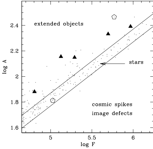
Fig. 6. F-A diagram for one of the images we analyzed (as an example). All the detected sources are plotted as small points. Filled triangles correspond to already confirmed clusters, empty pentagons to the candidate clusters under consideration. The continuous lines enclose the locus of point sources. Extended objects are expected to populate the upper left corner above the strip, while cosmic spikes and CCD cool/hot pixels must be confined to the lower right corner of the plot.
