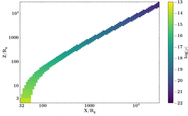
Figure A4. Colour map of an example model run showing the distribution of the mass number density through the wind cells that falls off with radius as a function of R^{(\kappa=-1)} . The corresponding density values in log scale are shown in the colour bar in units of \text{g cm}^{-3} . The x -axis represents the disc plane, while the z -axis is along the rotational axis. Both axes are in units of gravitational radii.
