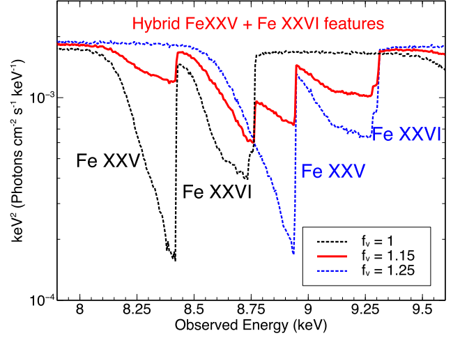
Figure 11. Three simulated microcalorimeter resolution (i.e. 2 eV at 6.4 keV) spectra, using a high-resolution f32hires grid, corresponding to f_v = 1 (black) and f_v = 1.25 (blue). The remaining disc-wind parameters are fixed to \Gamma = 2 , \mathcal{M}_w = 0.3 , \mathcal{L}_X = 0.5 , and \mu = 0.625 . The interpolated spectrum between f_v = 1 and f_v = 1.25 corresponding to f_v = 1.15 is shown in red. Note the asymmetry of the profiles visible at high resolution is a direct result of the acceleration of the gas along the streamline.
