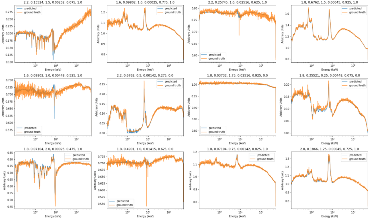
Figure 5. Randomly chosen examples of 12 ground truth spectra (orange) out of the 17280 available from the test data (10 per cent of total) with the corresponding emulated predicted spectra (blue). Note the ANN had not seen the spectra from the test set (10 per cent of the total) during training. The input parameters corresponding to \{\Gamma, \dot{\mathcal{M}}_w, f_v, \mathcal{L}_X, \mu, R_{\min} = 64 r_g (0.0) \text{ or } 32 r_g (1.0)\} are listed above each plot.
