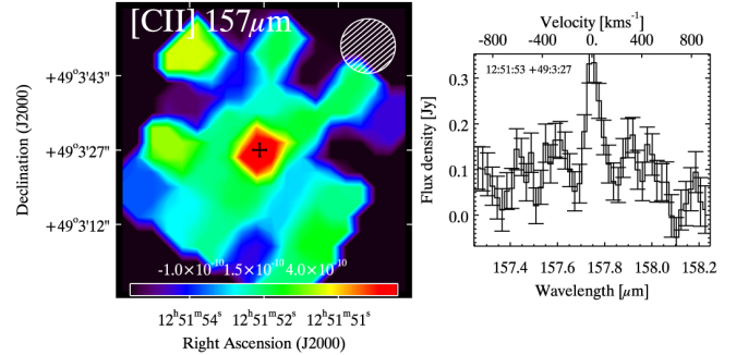
SBS1249+493
