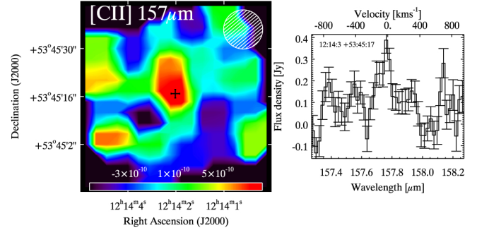
SBS1211+540
