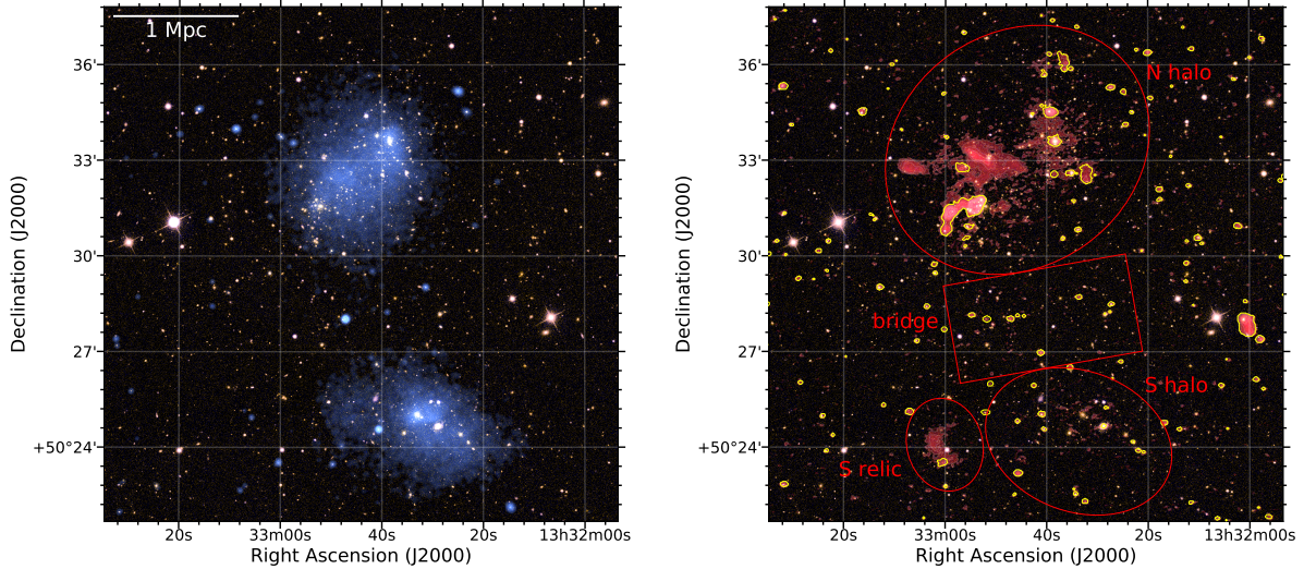
Figure 1. Composite images of A1758 obtained from the superposition of an optical SDSS g,r,i mosaic with Chandra (blue) and with a LOFAR image at 144 MHz with a resolution of 7.6'' \times 5.4'' (red) and a rms noise of 60 \mu\text{Jy beam}^{-1} . Yellow and red regions indicate the mask used to subtract discrete sources and the regions adopted to measure the flux densities in the low-resolution images, respectively.
