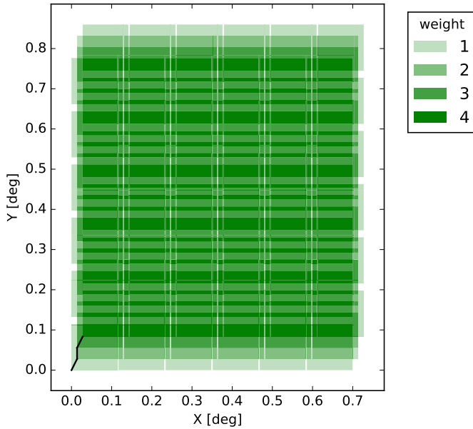
Fig. 2. Coverage of a single slew by VIS. The default dither pattern in Euclid is “S”-shaped (shown as the black lines in the bottom left corner) with displacements (\Delta x, \Delta y) = (0,0; 50,100; 0,100; 50,100) . The weights show the number of times an area has been observed. In each field of view there are 6 \times 6 non-square CCDs that have asymmetric spacing between them in the vertical and horizontal directions, which results in a non-square field of view.
