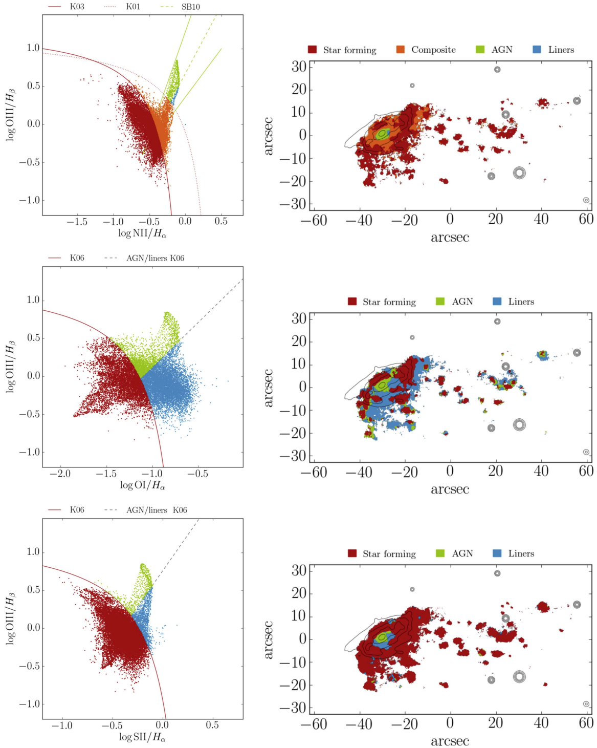
Figure 9. BPT line-ratio diagrams (left) and maps (right) for [O III] 5007/H \beta vs. [N II] 6583/H \alpha (top), vs. [O I] 6300/H \alpha (middle), and vs. [S II] 6717/H \alpha (bottom). Lines in the left panels are from Kauffmann et al. (2003, K03), Kewley et al. (2001, K01; 2006, K06), and Sharp & Bland-Hawthorn (2010, SB10) to separate star-forming, composite, the AGN, and LINERS. Contours are stellar isophotes, as in Figure 4.
