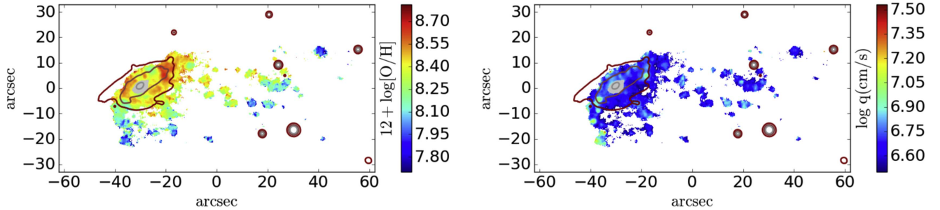
Figure 11. Metallicity (left) and ionization parameter (right) map. The central region powered by an AGN according to the BPT [N II] 6583/H \alpha diagnostic has been masked (gray area). Contours are stellar isophotes, as in Figure 4.
