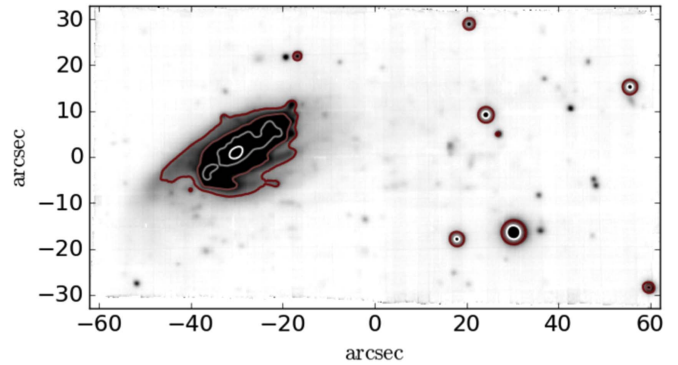
Figure 4. MUSE white image of JO206. Contours are logarithmically spaced isophotes of the continuum underlying H\alpha and thus are stellar isophotes down to a surface brightness 2.5 \times 10^{-18} \text{ erg s}^{-1} \text{ cm}^{-2} \text{ \AA}^{-1} \text{ arcsec}^{-2} . Round isolated contours are Galactic stars that are masked in the subsequent analysis. In this and all plots, (0, 0) is the center of the MUSE combined image. North is up and east is left.
