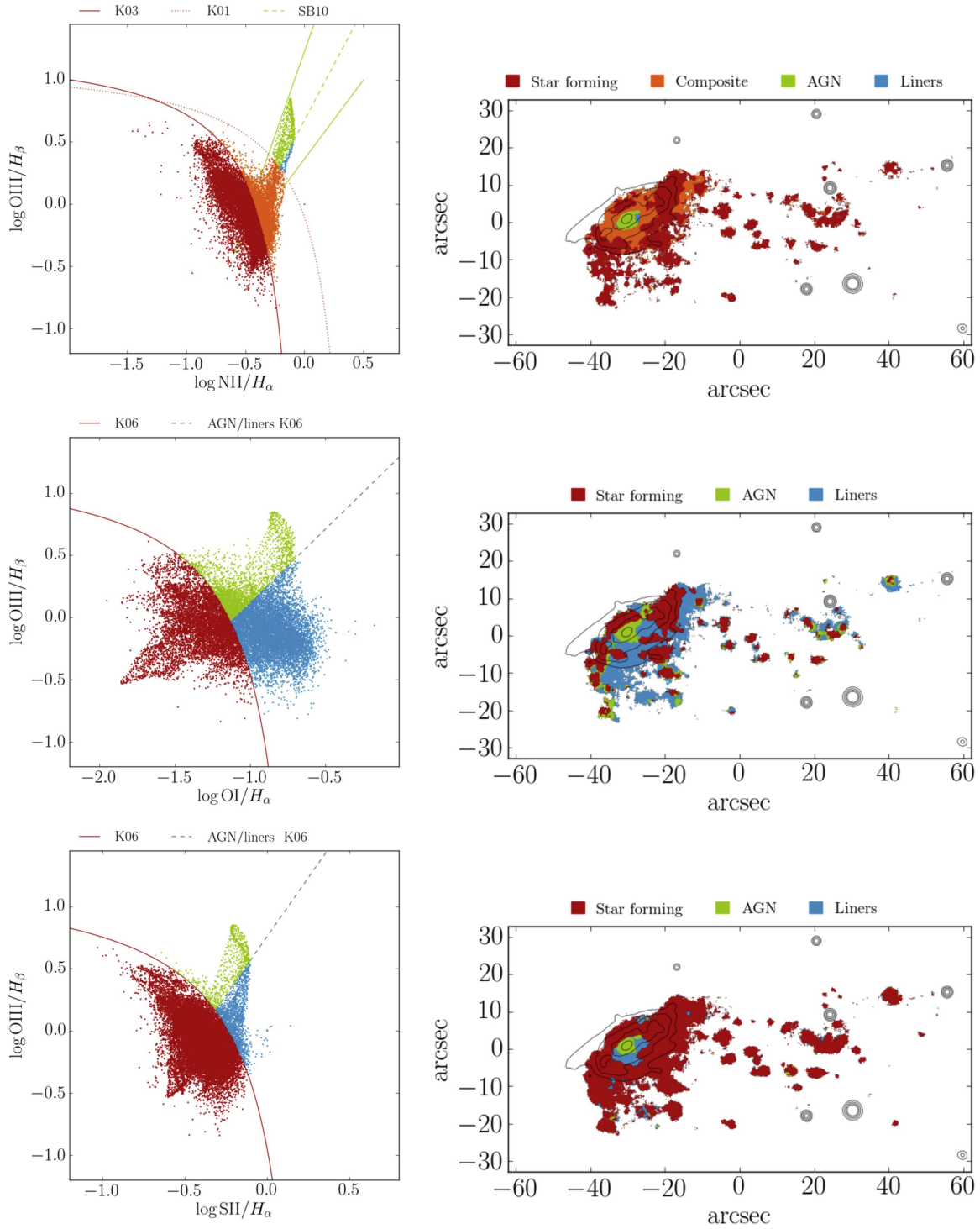
Figure 9. BPT line-ratio diagrams (left) and maps (right) for [\text{O III}] 5007/\text{H}\beta vs. [\text{N II}] 6583/\text{H}\alpha (top), vs. [\text{O I}] 6300/\text{H}\alpha (middle), and vs. [\text{S II}] 6717/\text{H}\alpha (bottom). Lines in the left panels are from Kauffmann et al. (2003, K03), Kewley et al. (2001, K01; 2006, K06), and Sharp & Bland-Hawthorn (2010, SB10) to separate star-forming, composite, the AGN, and LINERS. Contours are stellar isophotes, as in Figure 4.
