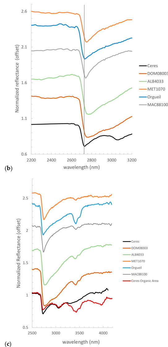
Figure 2. (a) Comparison between the spectra of Ceres and heated carbonaceous chondrites (Ceres from [24]; Heated carbonaceous chondrite (CC) from [31], SShade database). (b) Zoom in the region of the phyllosilicate absorptions. Comparison between the spectra of Ceres and heated carbonaceous chondrites (Ceres from [24]; heated CC from [31], SShade database). (c) Comparison between the spectra of Ceres (average-black spectrum, organic-rich region-red spectrum) and heated carbonaceous chondrites (Ceres from [24]; heated CC from [31], SShade database).
