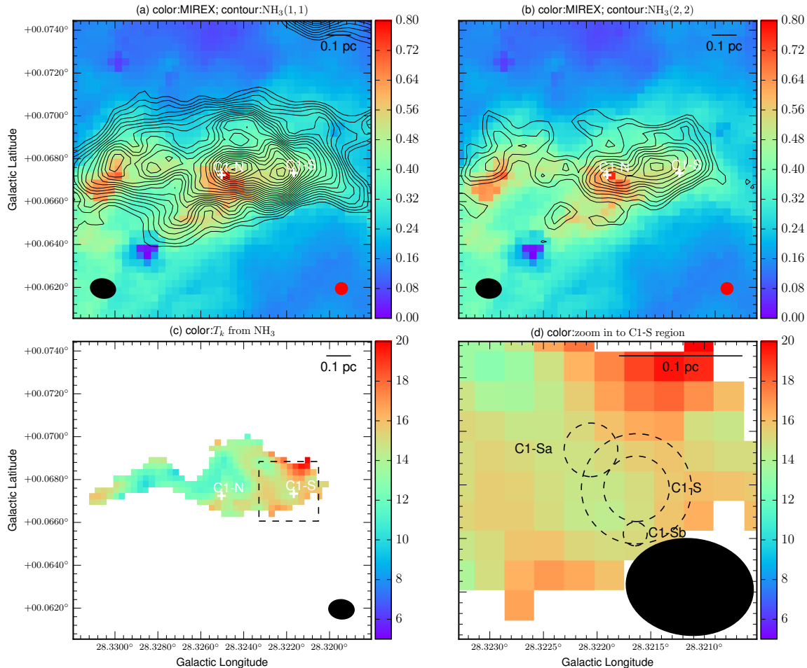
Figure 2. (a) Zeroth moment map of \text{NH}_3(1,1) integrated from 76.9 to 81.9 \text{km s}^{-1} (contours, shown from 3, 4, 5 \sigma , etc., with \sigma being 4 \text{mJy km s}^{-1} ). The integration covers the main hyperfine structure. The background image shows the MIR+NIR extinction map (in \text{g cm}^{-2} ) from Butler et al. (2014). The white plus signs represent the C1-N and C1-S cores from T13. The black circle in the lower-right shows the resolution beam of the extinction map. The black ellipse in the lower-left shows the synthesized beam of the VLA observations. (b) As panel (a), but now showing zeroth moment map of \text{NH}_3(2,2) . (c) T_k map derived from the VLA \text{NH}_3 observations. The color scale bar has the unit of K. The filled ellipse is the beam of the VLA observations. The dashed inset shows the zoom-in region of C1-S in panel (d). (d) Zoom-in view to the C1-S region in the T_k map. The black dashed circles represent the C1-S, C1-Sa and C1-Sb core definitions (see §3.1 and §3.2.1). The filled ellipse in the lower-right is the beam of the VLA observations.
