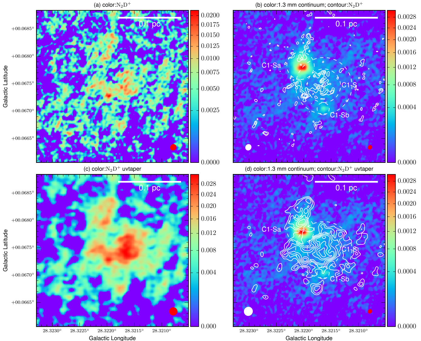
Figure 3. \text{N}_2\text{D}^+ observations: (a) Combined \text{N}_2\text{D}^+(3-2) 0th-moment map. The integration is from 76.9 to 81.9 \text{km s}^{-1} (i.e., centered on 79.4 \text{km s}^{-1} velocity measured by T13). The color scale bar has a unit of \text{Jy beam}^{-1} \text{ km s}^{-1} . The synthesized beam ( \sim 0.3'' ) is shown as a red filled ellipse at lower-right. (b) \text{N}_2\text{D}^+(3-2) 0th-moment contours overlaid on the 1.3 mm continuum image. The continuum image and color scheme is the same as Figure 1c. The \text{N}_2\text{D}^+(3-2) contours start from 3\sigma and increase in step of 1\sigma ( \sigma = 3 \text{ mJy km s}^{-1} ). The red filled ellipse at lower-right is the synthesized beam for the continuum image. The white filled ellipse at lower-left is the beam for the \text{N}_2\text{D}^+(3-2) contour map. The dashed circles are the core definitions for C1-Sa, C1-Sb, “C1-S inner” and “C1-S outer.” (c) Same as (a), but now the \text{N}_2\text{D}^+(3-2) 0th-moment map is uv-tapered to \sim 0.5'' resolution. (d) Same as (b), but now the \text{N}_2\text{D}^+(3-2) 0th-moment contour map is uv-tapered to \sim 0.5'' resolution.
