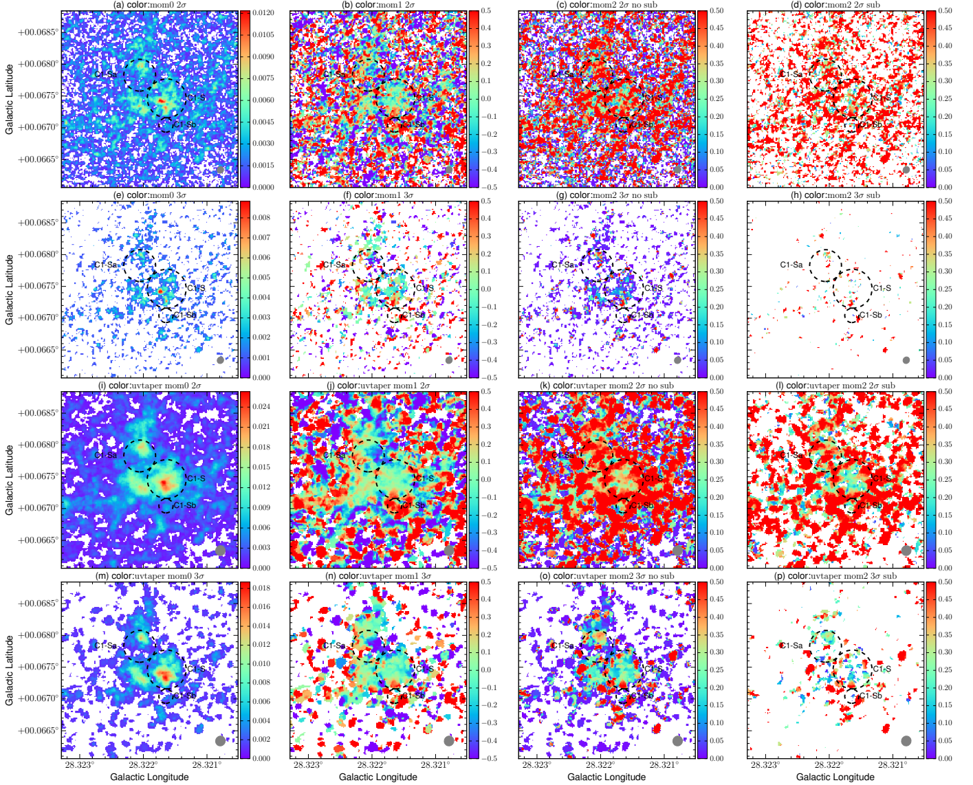
Figure 9. N_2D^+(3-2) moment maps. Columns from left to right: 0th-moment, 1st-moment (relative to 79.4 \text{ km s}^{-1} ), 2nd-moment without intrinsic dispersion subtraction, and 2nd-moment with the N_2D^+(3-2) hyperfine structure dispersion subtracted. Rows from top to bottom: combined data with 2\sigma cut, combined data with 3\sigma cut, uv-tapered data ( 0.5'' ) with 2\sigma cut, and uv-tapered data with 3\sigma cut. All moment calculations are carried out within the velocity range 79.4 \pm 1.5 \text{ km s}^{-1} to avoid any contribution from the 81.2 \text{ km s}^{-1} component. The subtraction of the intrinsic dispersion of 0.242 \text{ km s}^{-1} from the N_2D^+(3-2) hyperfine structure in the 4th column limits the number of available pixels in the final image. The beam is shown as the gray filled ellipse on the lower-right corner. The color bars for the 1st column have the unit \text{Jy beam}^{-1} \text{ km s}^{-1} , for the rest columns \text{km s}^{-1} .
