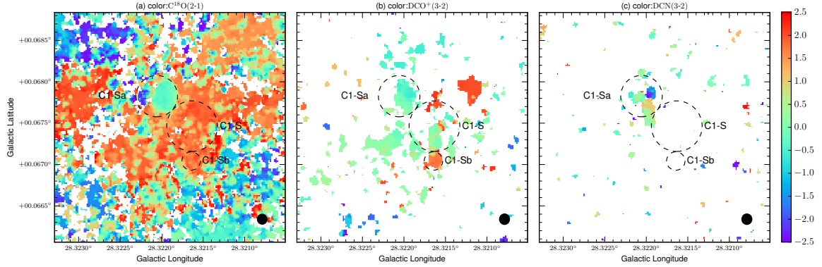
Figure 14. From left to right: 1st-moment maps of C^{18}O(2-1) , DCO^+(3-2) and DCN(3-2) . The integration is over 79.4 \pm 2.5 \text{ km s}^{-1} . Only cells above 3\sigma are considered. The 1st-moment is then normalized to the rest frame of 79.4 \text{ km s}^{-1} . The beams are shown as the black filled ellipses in the lower-right corners. The colorbar has the unit \text{km s}^{-1} .
