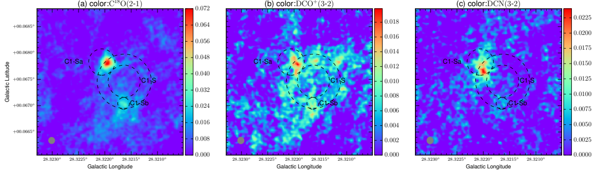
Figure 13. From left to right: 0th-moment maps of C^{18}O(2-1) , DCO^+(3-2) and DCN(3-2) . All panels show the combined data. The integrations are from 76.9 to 81.9 \text{km s}^{-1} . The color scale bars have unit of \text{Jy beam}^{-1} \text{km s}^{-1} . The synthesized beams ( \sim 0.3'' ) are shown as gray filled ellipses in the lower-left corners.
