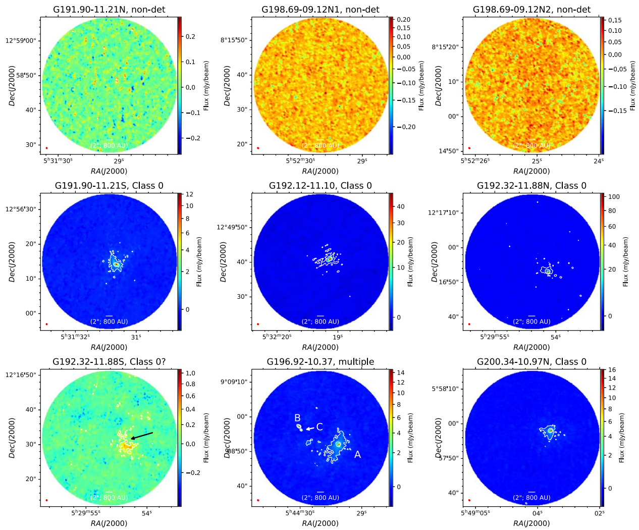
Figure A1. \lambda -Orionis: Combined TM1, TM2, and 7 m ACA continuum images of nondetected dense cores and Class 0 systems (including multiples). Contours are at 6 and 30\sigma , where the corresponding \sigma s are tabulated in Table 1.
