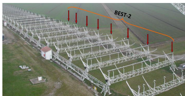
Figure 4. BEST-2 antennas
