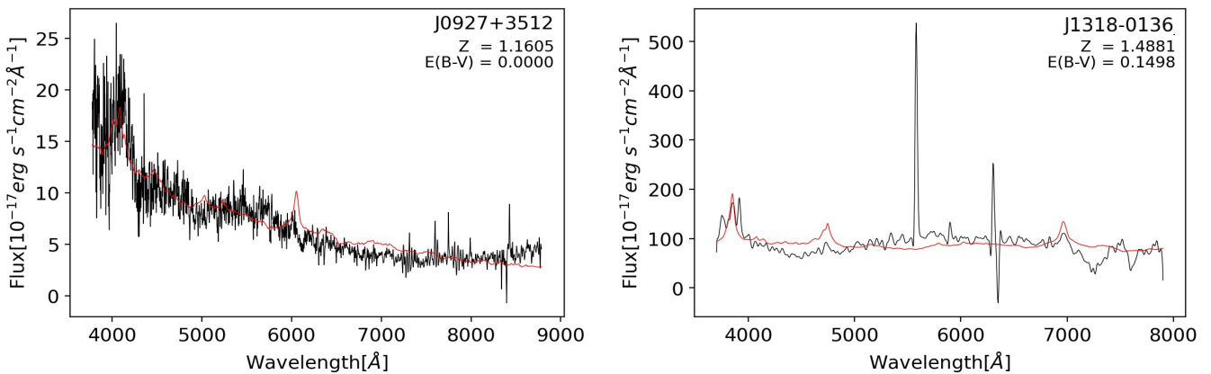
Fig. A.3. Spectral deconvolution of the unclassified objects, i.e., the systems whose spectra are not well reproduced from an AGN or from an AGN plus a star.
