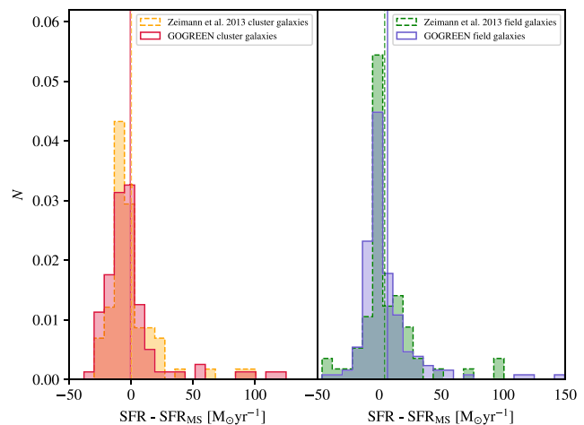
Figure B1. [O II]-derived GOGREEN cluster (solid) \Delta\text{SFR}_{\text{MS}} distribution and H \alpha -derived Zeimann et al. (2013) cluster (dashed) \Delta\text{SFR}_{\text{MS}} distribution (left). GOGREEN field (solid) and Zeimann et al. (2013) field (dashed) \Delta\text{SFR}_{\text{MS}} distributions are shown on the right.
