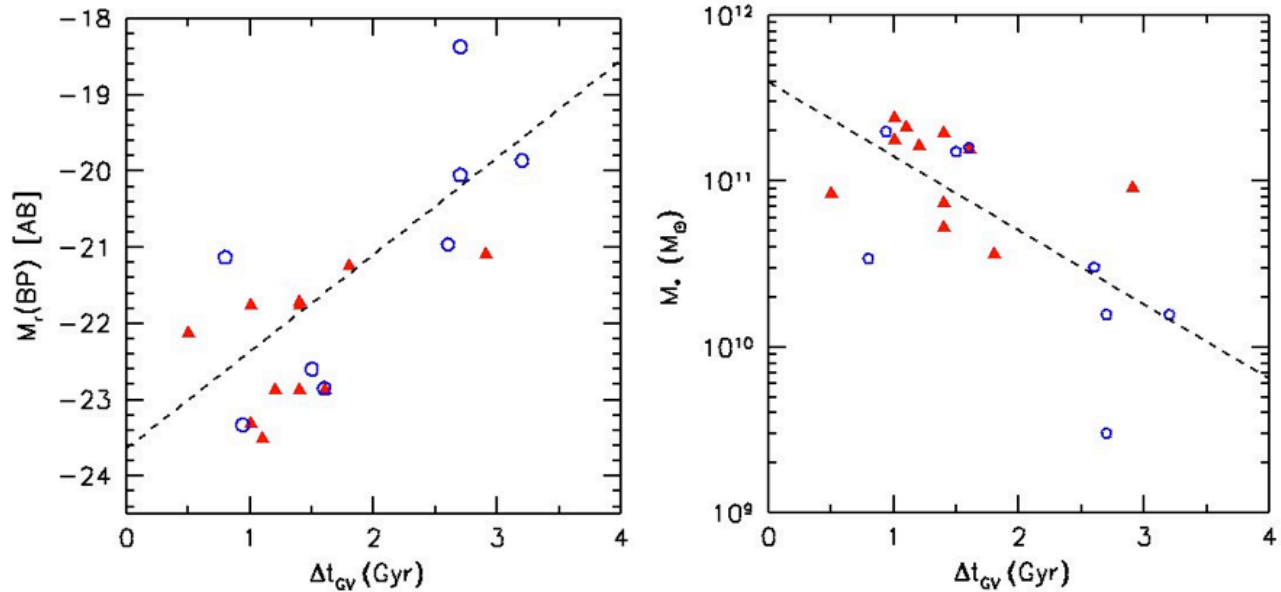
Figure 8. ( Left ) The absolute M_r magnitude reached at the Brightest Point of the rest-frame CMD diagram vs. the time spent in the GV, as defined in Section 4; the correlation (dashed line) index is 0.72, and the slope of the regression is 1.27. ( Right ) The total stellar mass at z=0 vs. the time spent in the GV; the correlation (dashed line) index is -0.67, and the slope of the regression is -0.45. Symbols are as in Fig.7.
