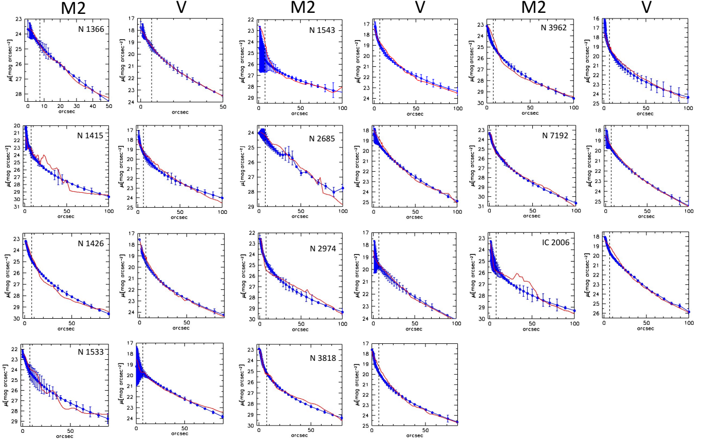
Figure 3. Luminosity profiles of our targets in the Swift -UVOT M2 and V bands; blue dots are Sérsic functions in Paper II, red solid lines are from the simulation snapshots in Fig.2.
